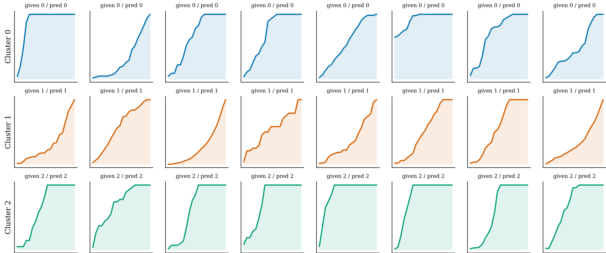
Case study: test-set trajectories with given (k-means) vs predicted (ft_transformer) labels test accuracy 99.99% — red title/border = misclassified
