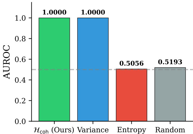
Hallucination Detection AUROC
