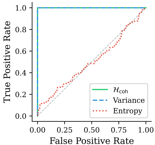
ROC Curves (n=400)
