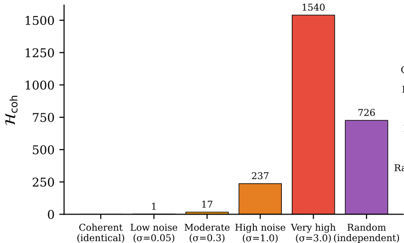
Cohomological Incoherence \mathcal{H}_{\text{coh}} vs. Noise Level
