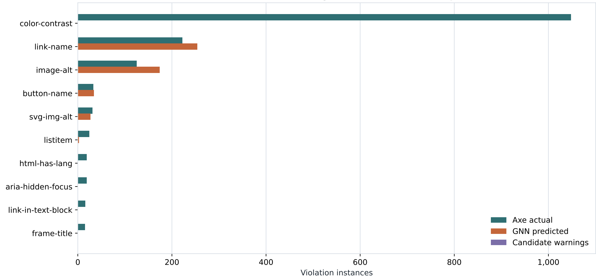
Rule distribution: axe ground truth vs GNN output
