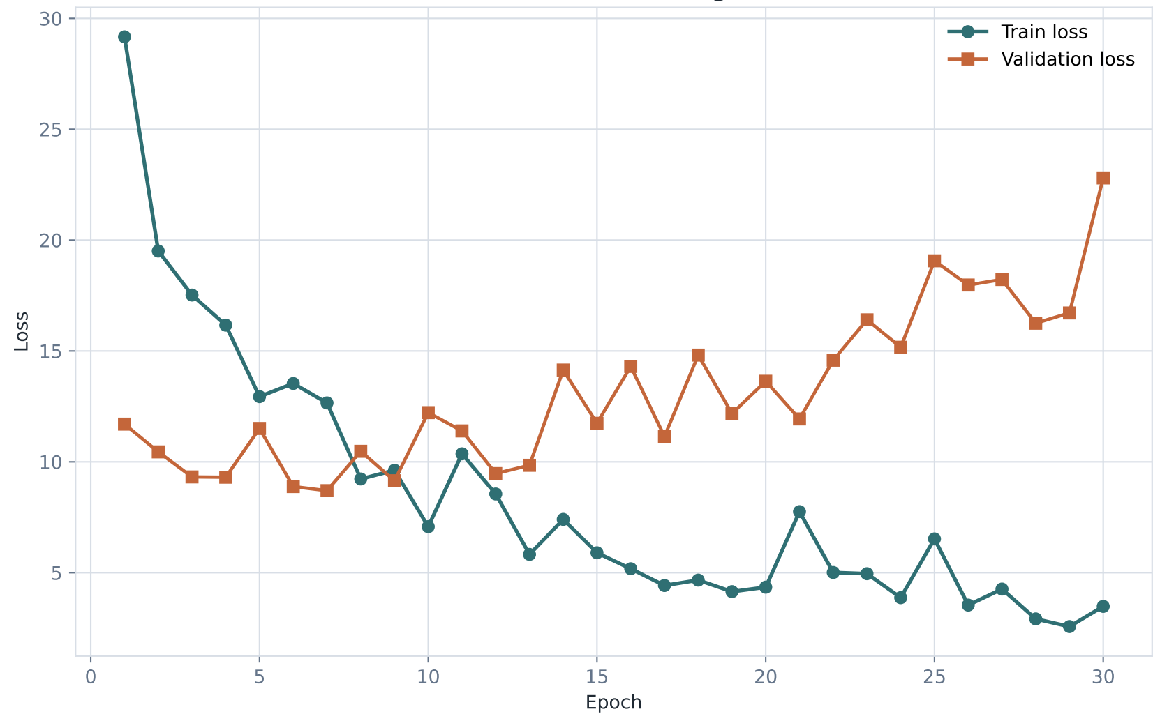
Loss over training
