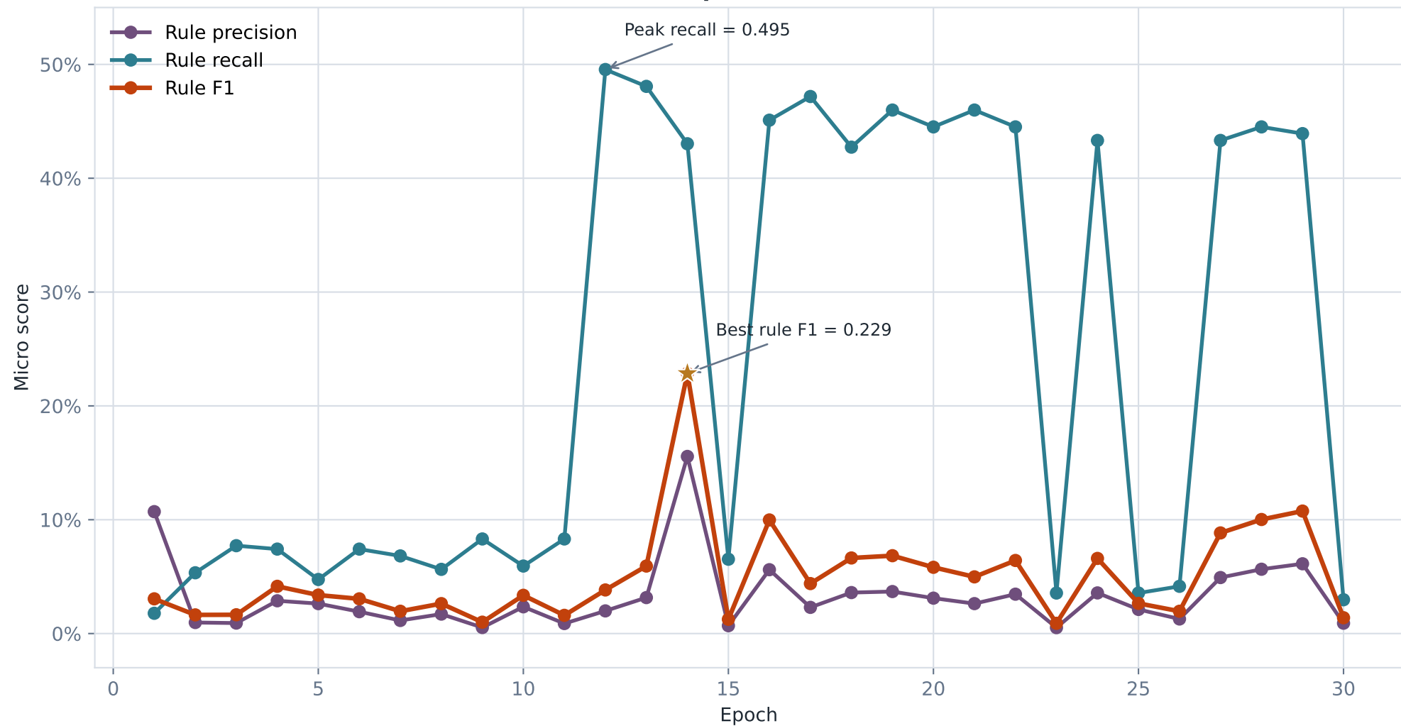
Rule-level micro precision, recall, and F1
