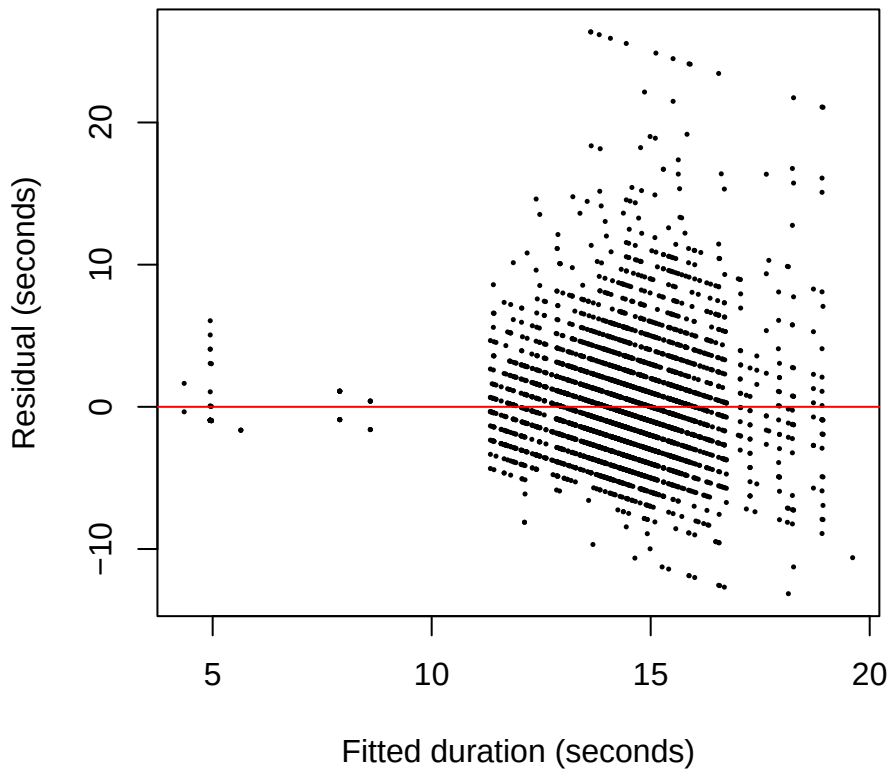
Residuals versus fitted
