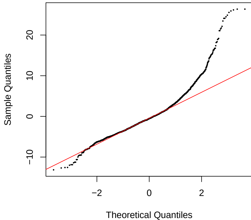
Residual Q-Q plot
