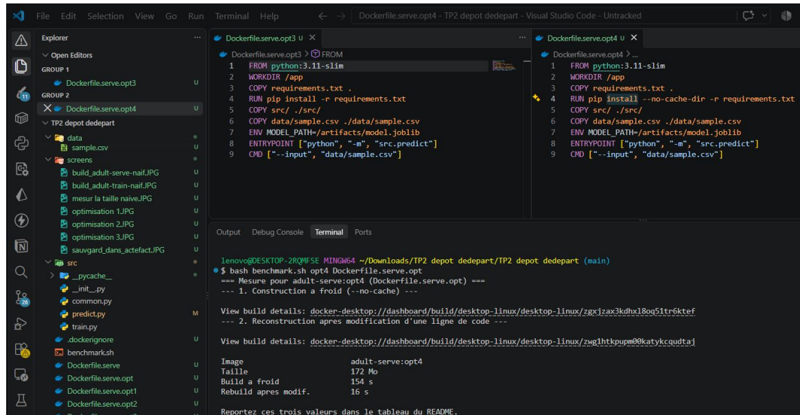
FIGURE 8 – Optimisation 4 — --no-cache-dir
