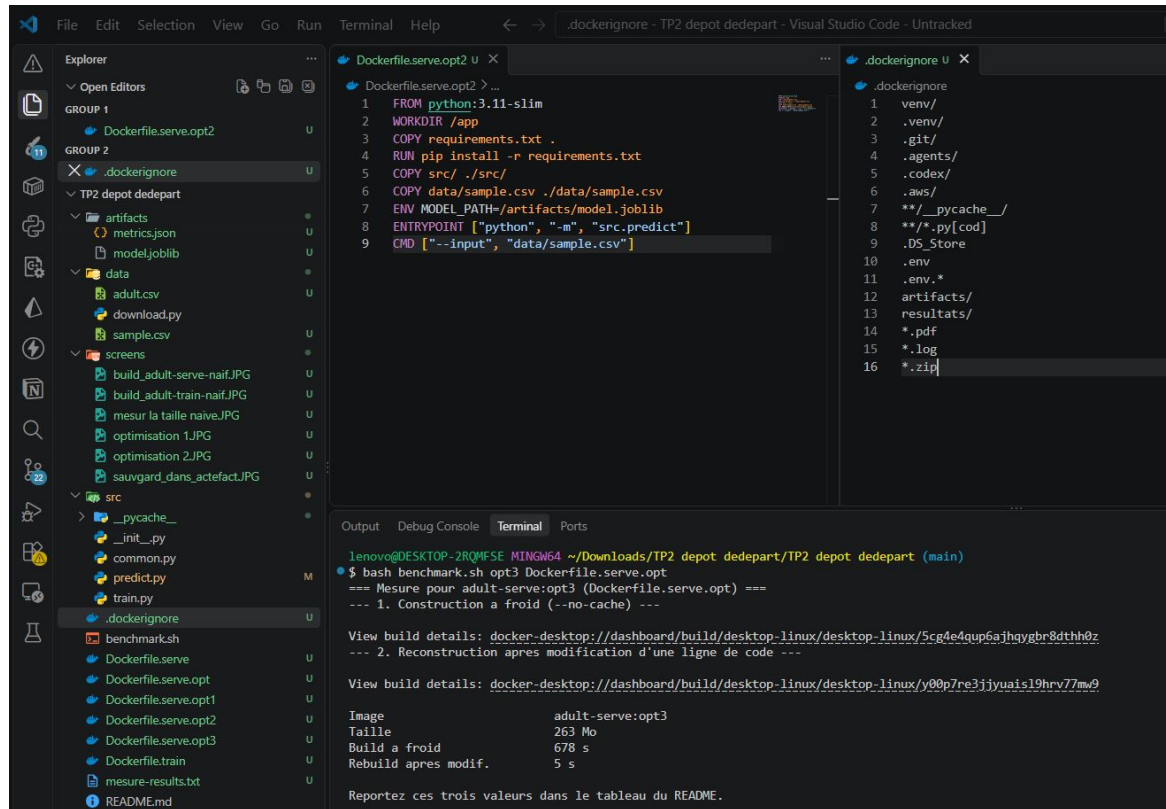
FIGURE 7 – Optimisation 3 — .dockerignore
