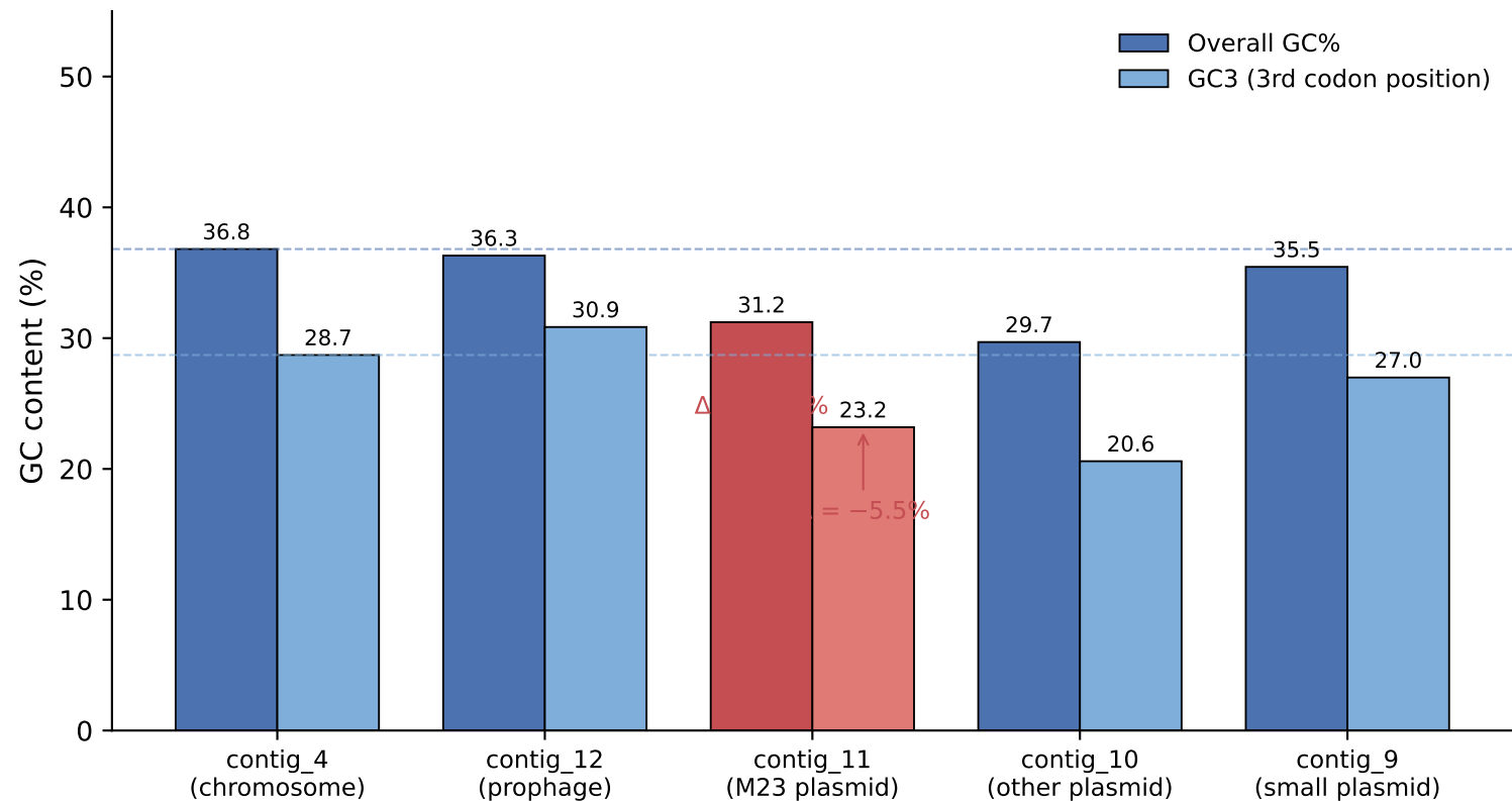
Per-contig GC and GC3 content of V. salarius PL25 (dashed lines: chromosomal baseline)
