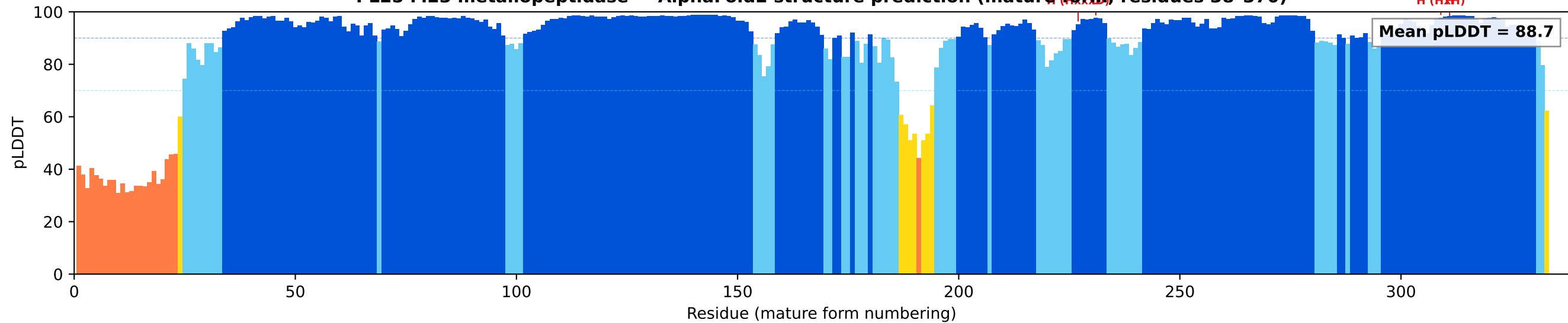
PL25 M23 metallopeptidase — AlphaFold2 structure prediction (mature form, residues 38-370)
