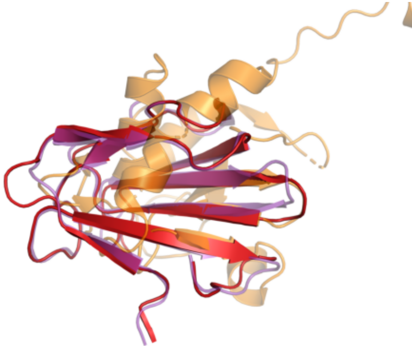
A — M23 catalytic domain only
