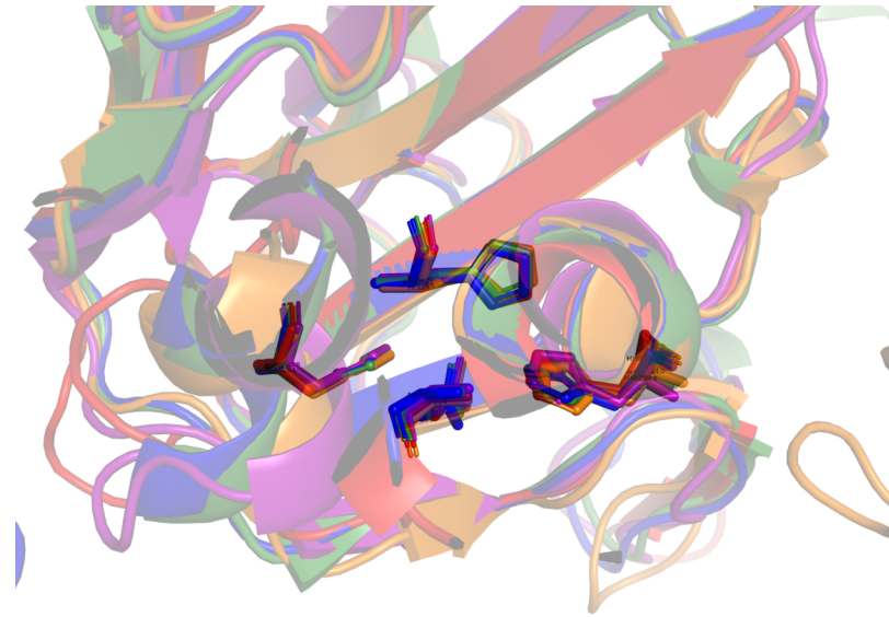
a Overlay of M23 catalytic-site residues — all five proteins superposed on PL25_M23 (residues 205-330)
