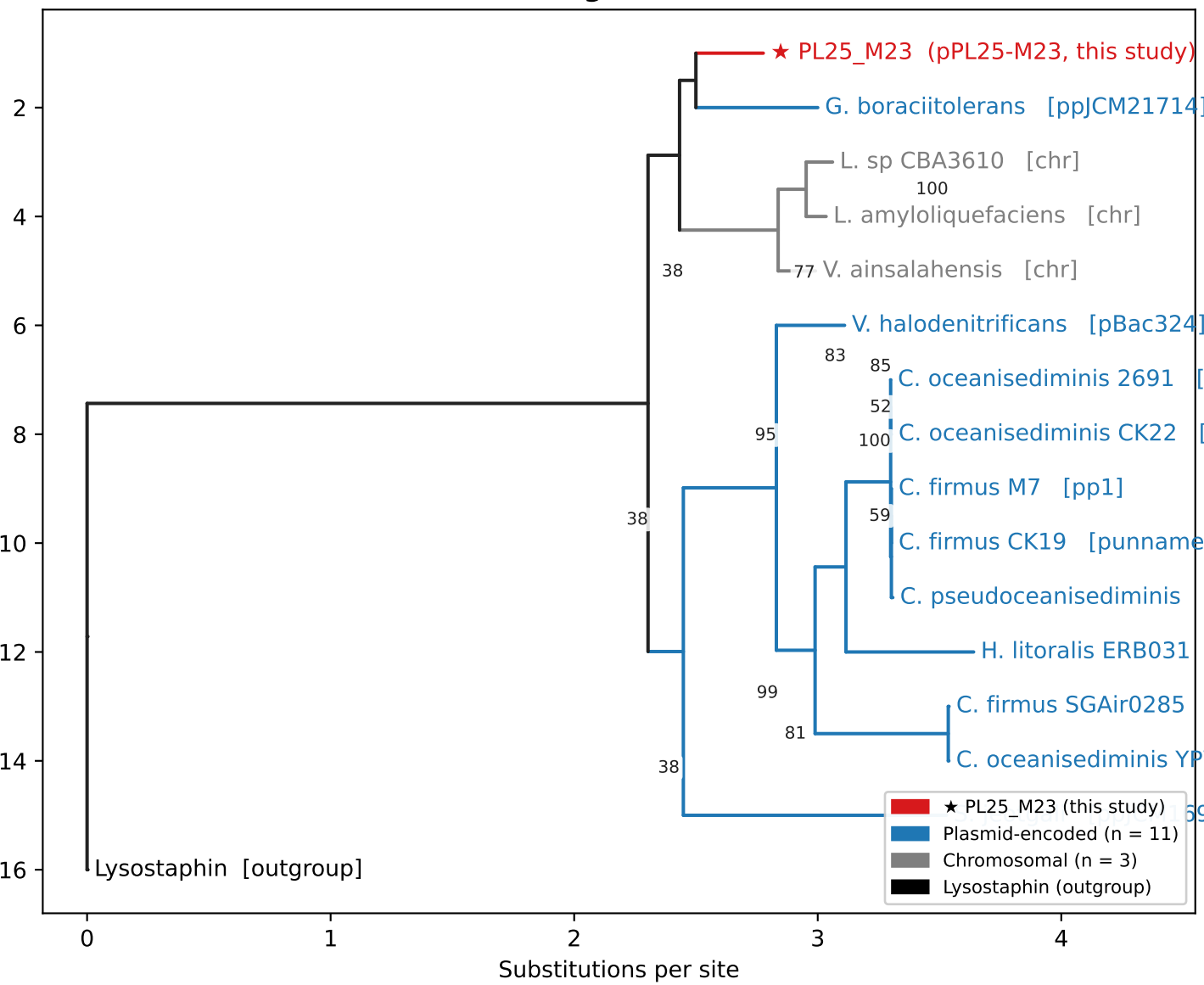
a Focused phylogeny of PL25_M23 and 14 closed-genome halotolerant Bacillaceae homologues
