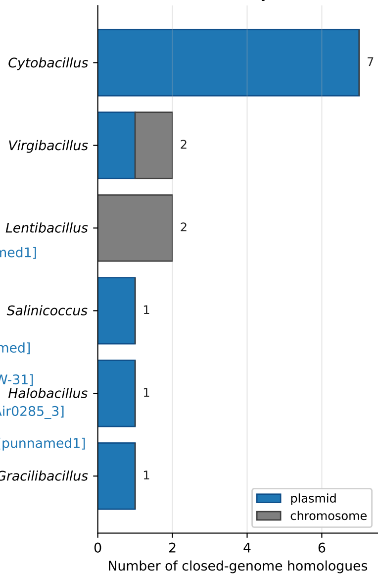
b Replicon context across genera (11 of 14, 79% plasmid-encoded)
