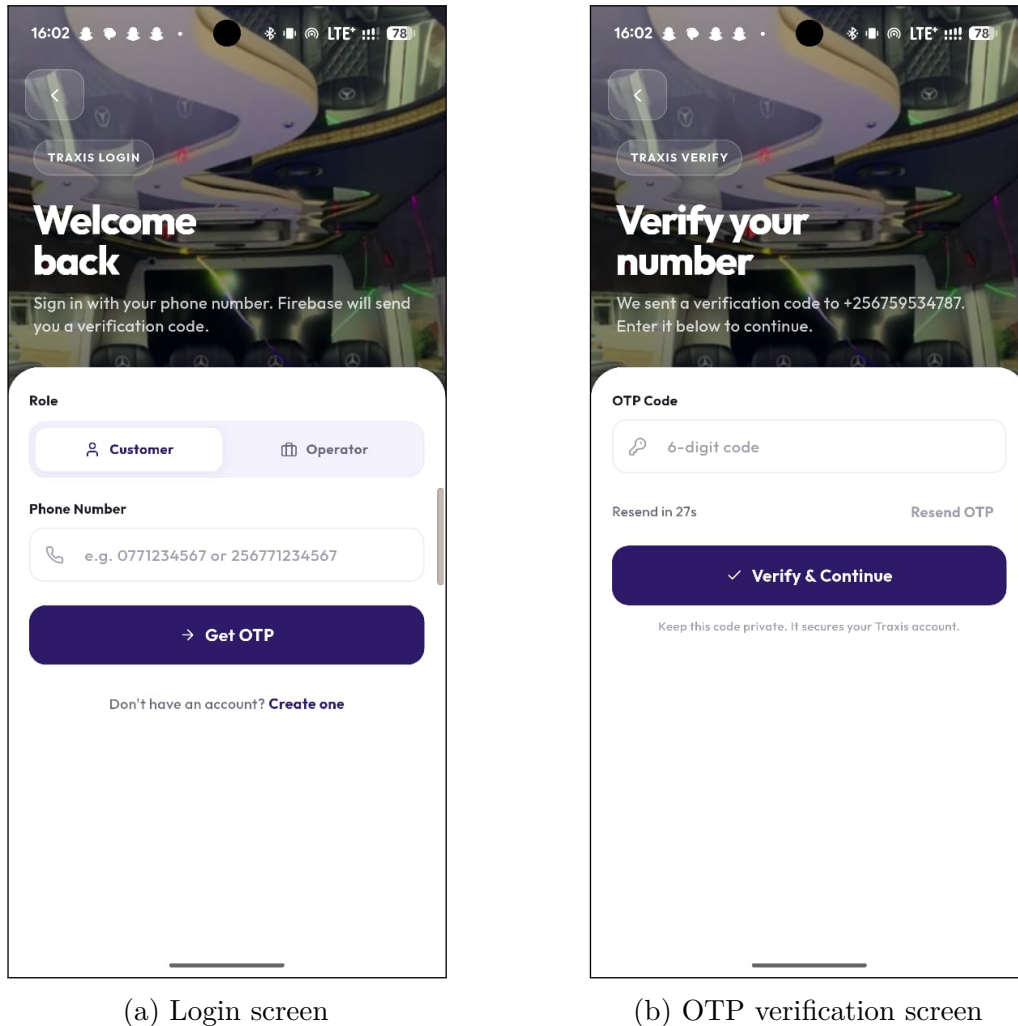
Figure 5.2: Authentication interfaces
