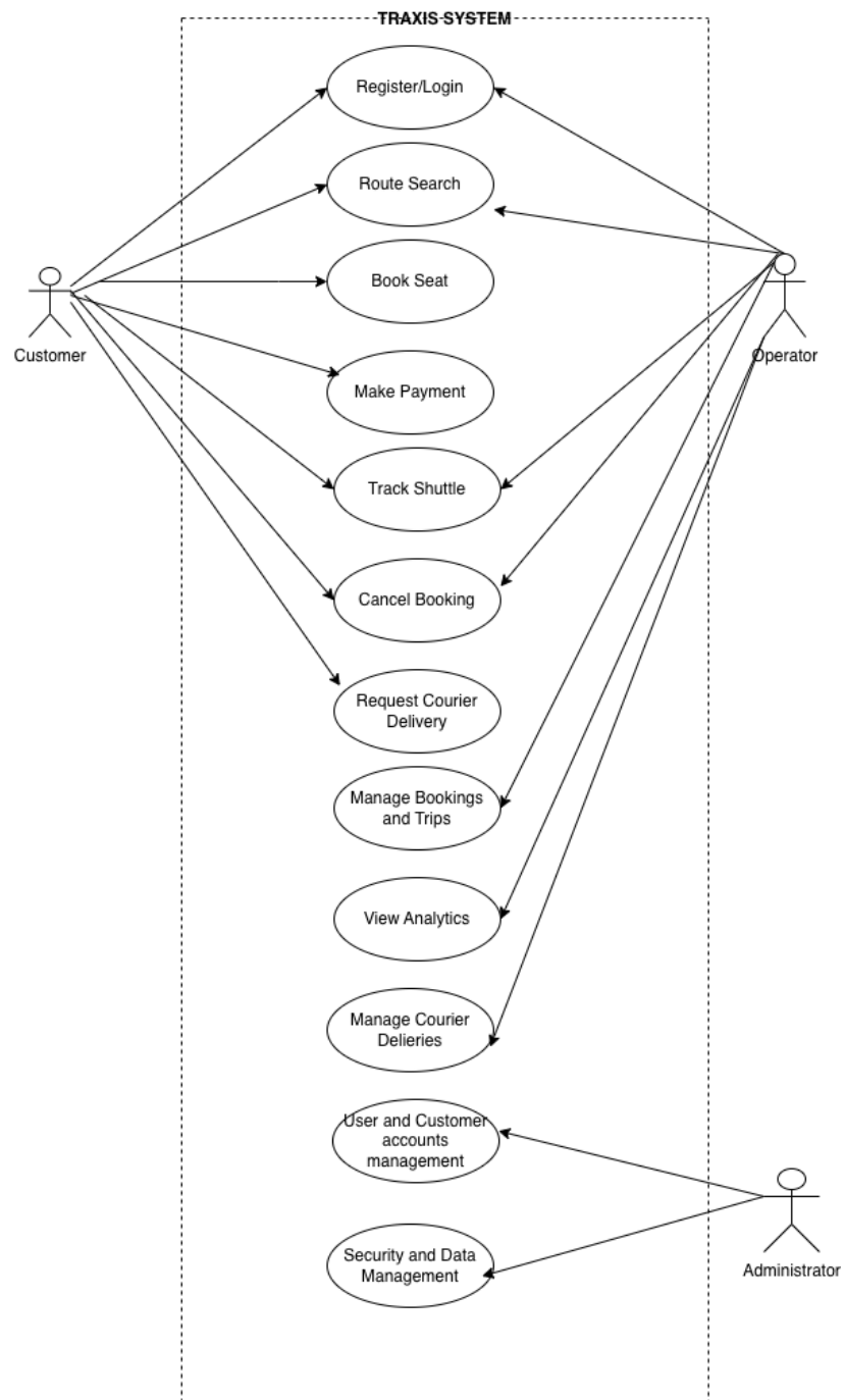
Figure 4.2: Use case diagram showing how users interact with the Traxis system
