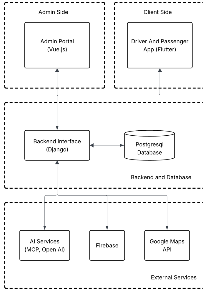
Figure 4.1: High-level system architecture of the TRAXIS platform
