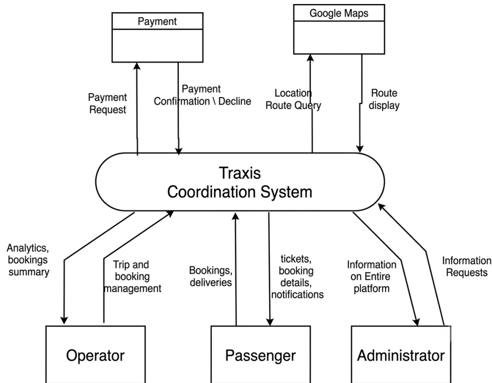
Figure 4.3: Level 0 Context Diagram showing the overall system boundary and external entities
