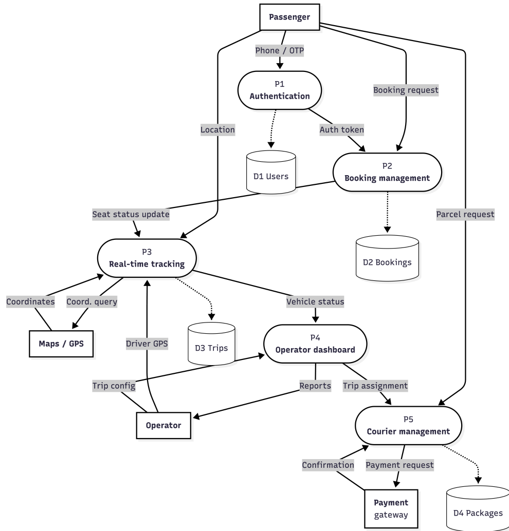
Figure 4.4: The Level 1 diagram decomposes the system further, revealing the core internal processes, data stores, and information flows between passengers, operators, and the Traxis platform.
