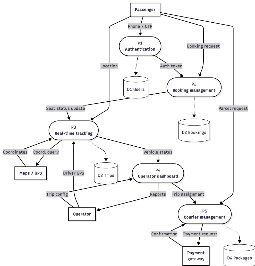
Figure 4.3: The Level 1 diagram decomposes the system further, revealing the core internal processes, data stores, and information flows between passengers, operators, and the Traxis platform.
