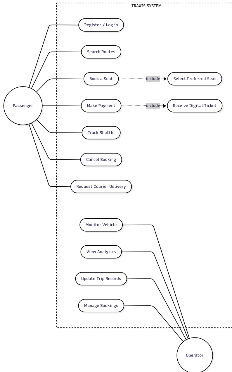
Figure 4.1: Use case diagram showing how users interact with the Traxis system
