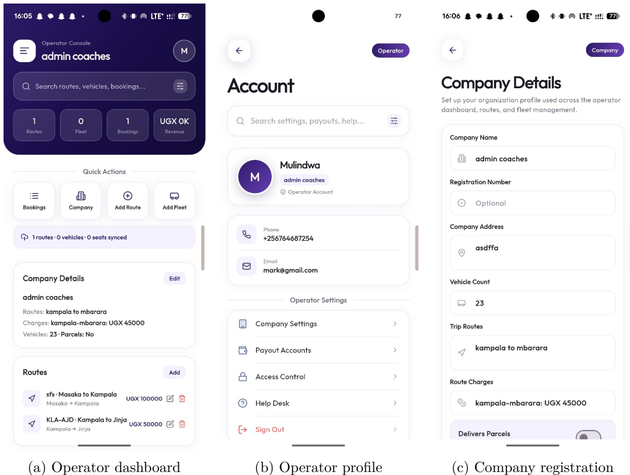
Figure 5.2: Operator interfaces
