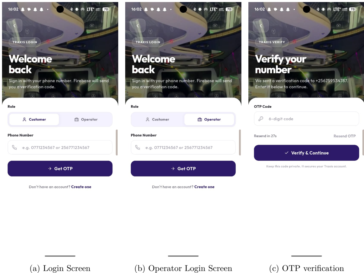
Figure 5.1: Authentucation interfaces
