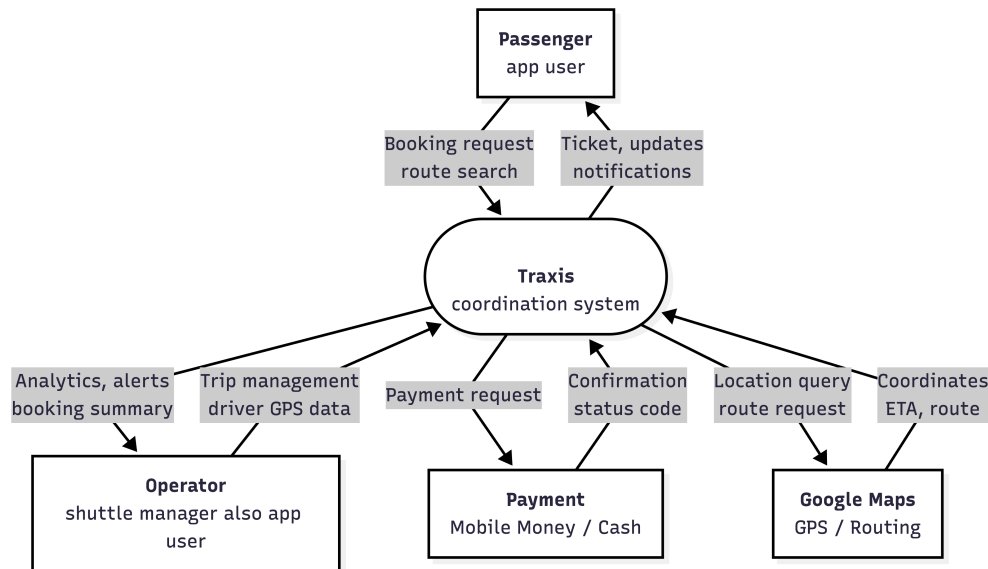
Figure 4.2: Level 0 Context Diagram showing the overall system boundary and external entities
