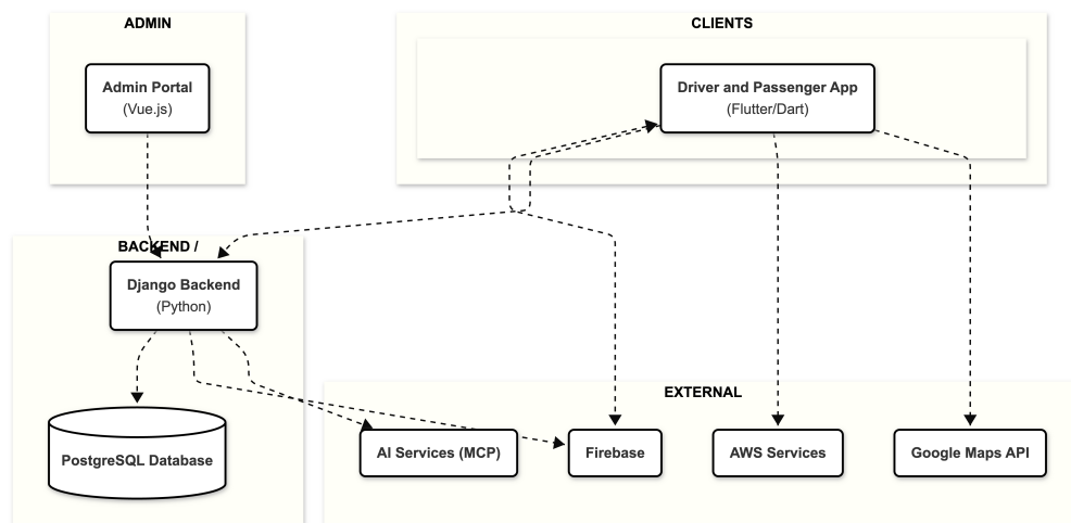
Figure 3.1: Methodology diagram of the entire system flow
