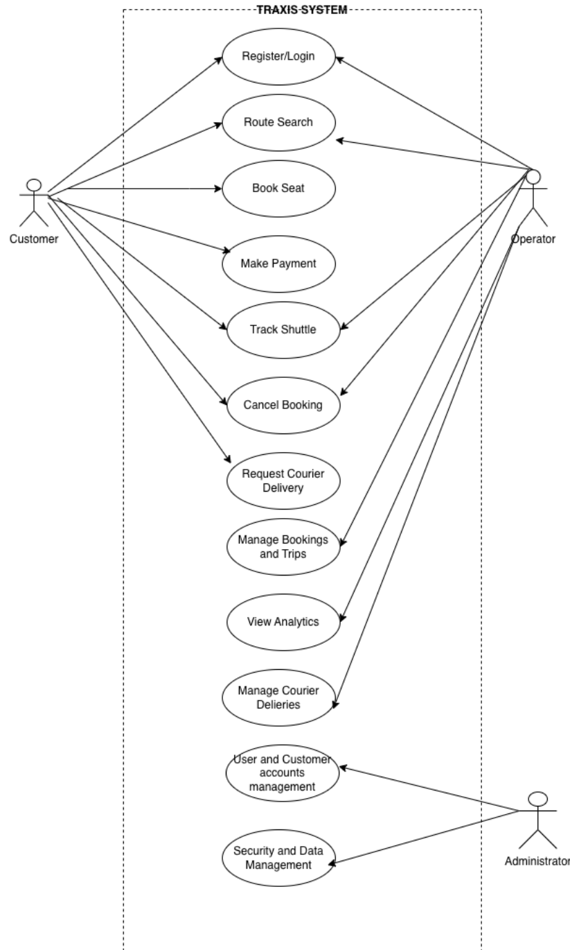
Figure 4.1: Use case diagram showing how users interact with the Traxis system
