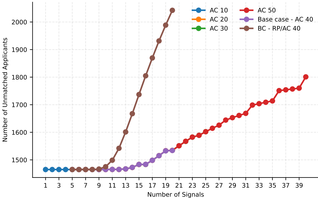
Number of Unmatched Applicants vs Number of Signals
