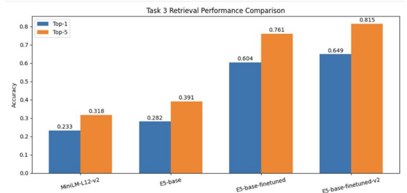
Figure 12: Model Retrieval Performance Comparison.
