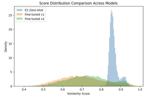
Figure 16: Score Distribution Comparison
