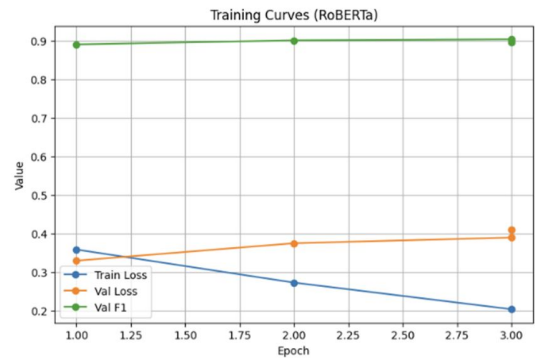
Figure 8: Training and validation loss curves across epochs.
