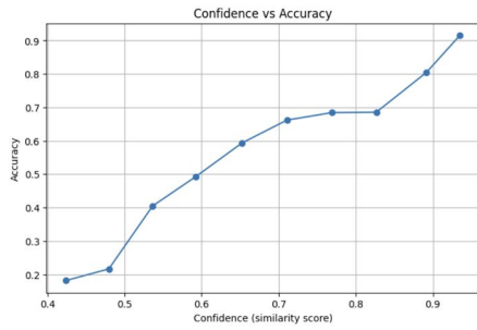
Figure 14: Confidence vs accuracy across similarity bins
