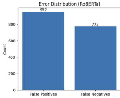
Figure 9: Error distribution (false positives vs false negatives).
