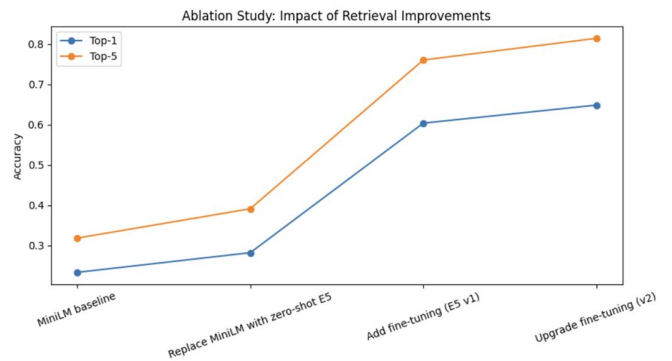
Figure 17: Ablation study: Impact of Retrieval Improvement
