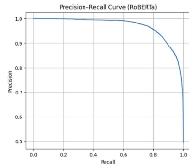
Figure 11: Precision–Recall curve for RoBERTa.
