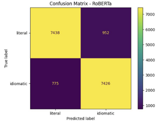
Figure 10: Confusion matrix for RoBERTa on the test set.
