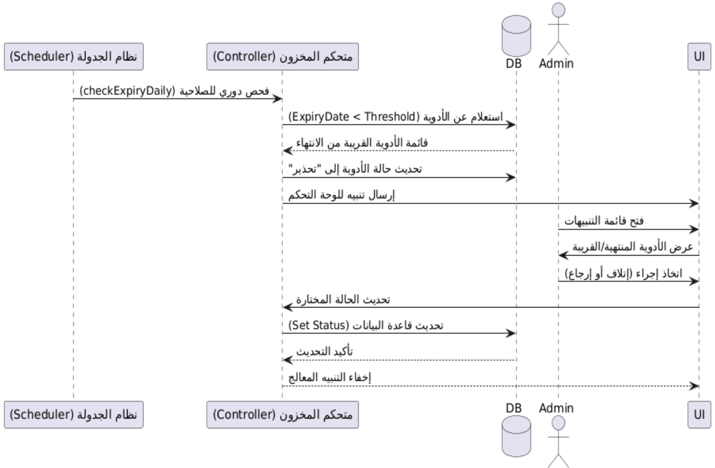
Sequence Diagram: Manage Expiry Alerts (Automatic & Manual)
