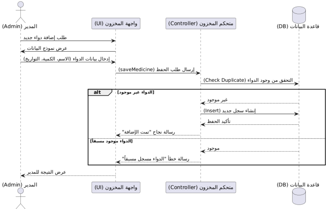
Sequence Diagram: Add New Medicine
