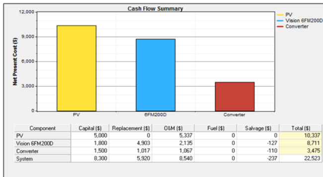
Figure 7: Cash flow summary of PV pumping system.
