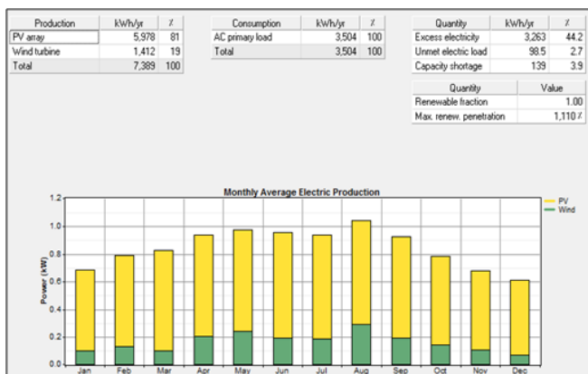
Figure 12: Energy summary of PV/HAWT pumping system.
