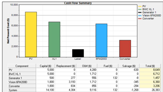
Figure 15: Cash flow summary of PV/HAWT/Diesel pumping system.
