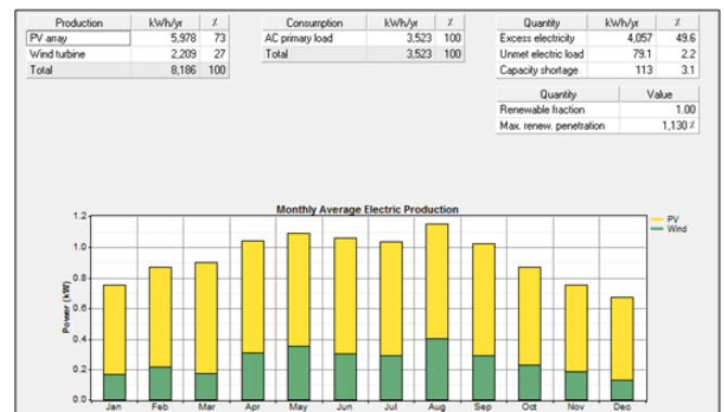
Figure 14: Energy summary of PV/VAWT pumping system.
