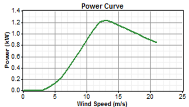
Figure 9: Wind turbine power curve.
