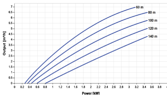
Figure 6: Solar pump chart.
