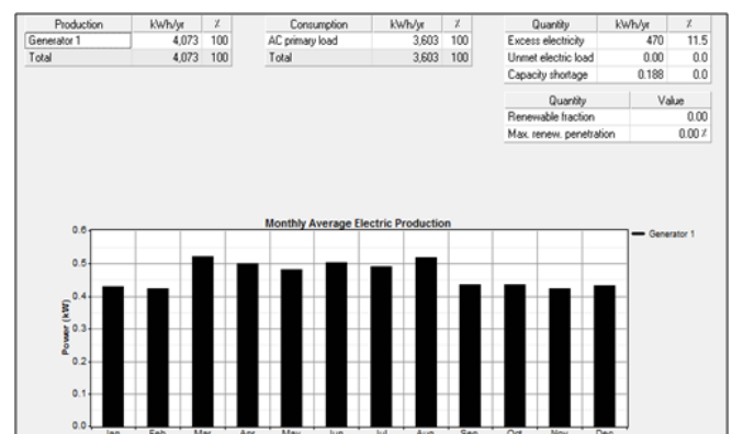
Figure 18: Energy summary of Diesel pumping system.
