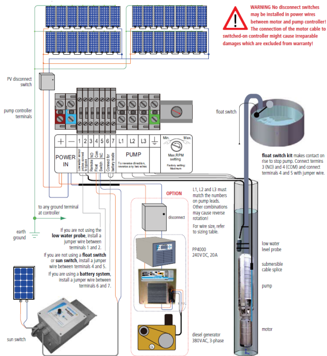
Figure 5: Wiring diagram of the pump controller.
