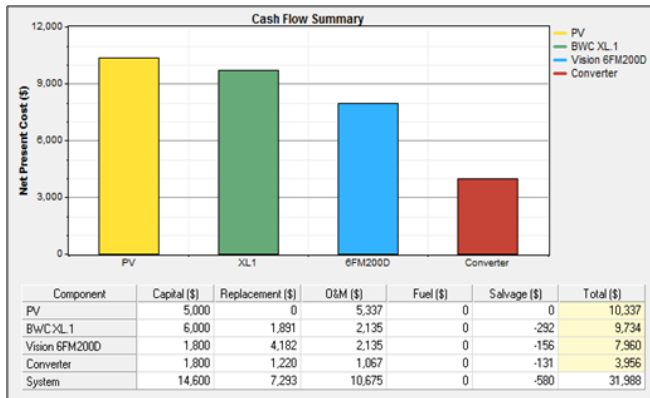
Figure 10: Cash flow summary of PV/HAWT pumping system (25 years).
