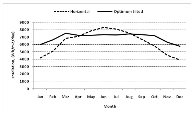
Figure 2: Irradiation levels on a horizontal and an optimally tilted surface in El-Tour, Sinai.
