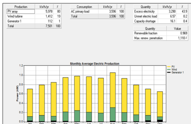
Figure 16: Energy summary of PV/HAWT/Diesel pumping system.
