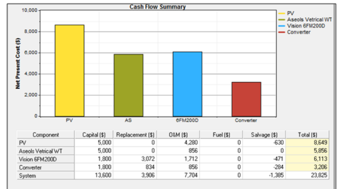
Figure 13: Cash flow summary of PV/VAWT pumping system.
