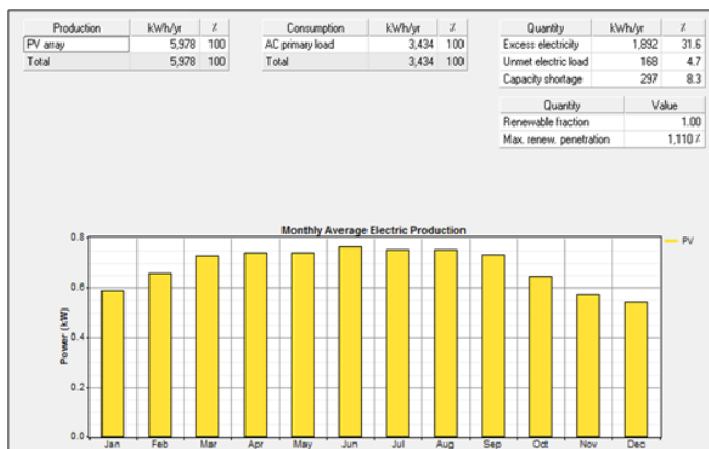
Figure 8: Energy summary of PV pumping system.
