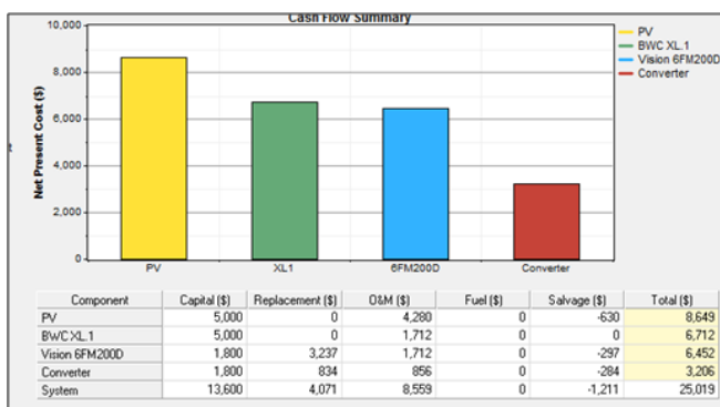
Figure 11: Cash flow summary of PV/HAWT pumping system (15 years).
