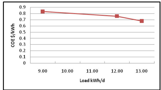
Figure 18: Relation between daily load and cost of energy (COE)
