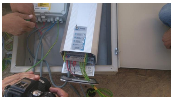
Figure 4: Pump controller.
