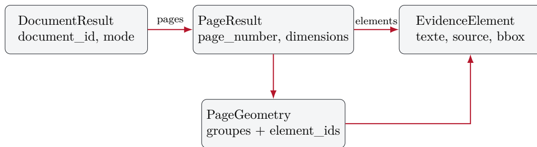
FIGURE 4.4 – Relations principales du contrat Document Intelligence.
