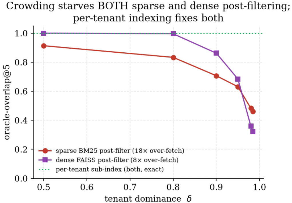
Figure 5: Measured: crowding starves both sparse (BM25, 18× over-fetch) and dense (FAISS, 8× over-fetch) post-filtering as tenant dominance rises; the per-tenant sub-index restores both to overlap 1.0.
