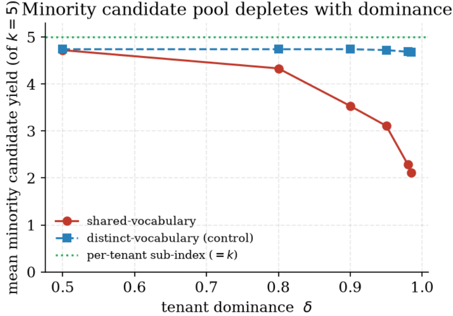
Figure 3: Figure 3: The minority candidate pool (yield of k=5 ) depletes with dominance for shared-vocabulary queries.
