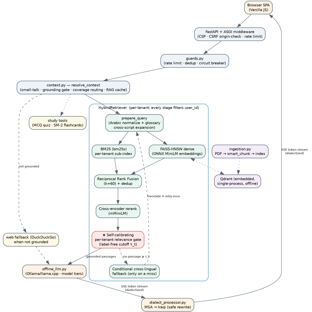
Figure 1: Figure 1: The retrieval pipeline (a query’s path through the system). Both the sparse (BM25) and dense (FAISS) paths filter by tenant; the per-tenant BM25 sub-index of this paper sits at the “BM25 (bm25s) per-tenant sub-index” node. The relevance gate and cross-lingual fallback are companion mechanisms (cited, not contributed here).
