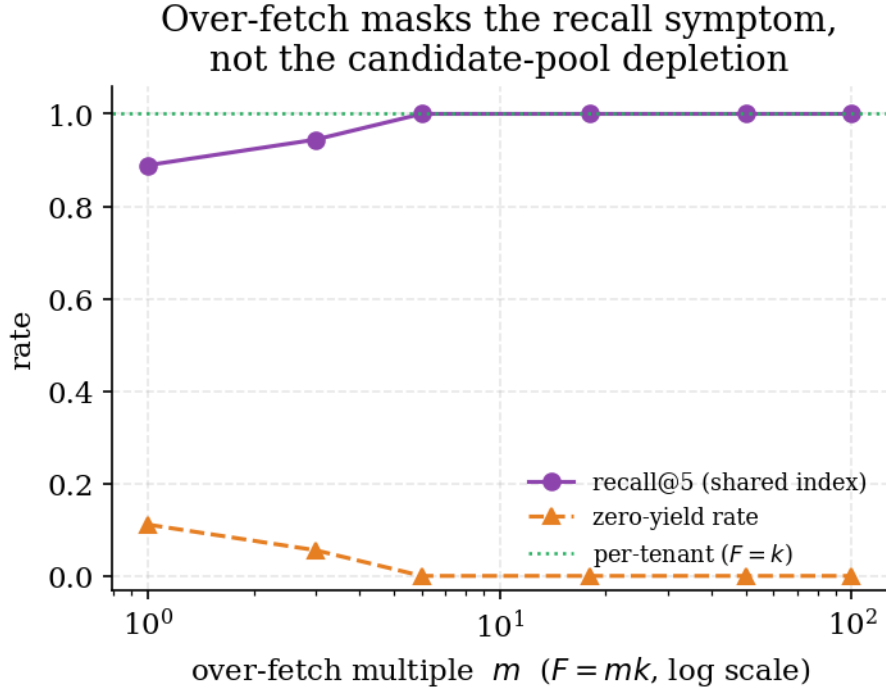
Figure 4: Figure 4: Over-fetch raises target recall (and removes zero-yield) but does not restore the candidate-pool depletion of Figure 3.
