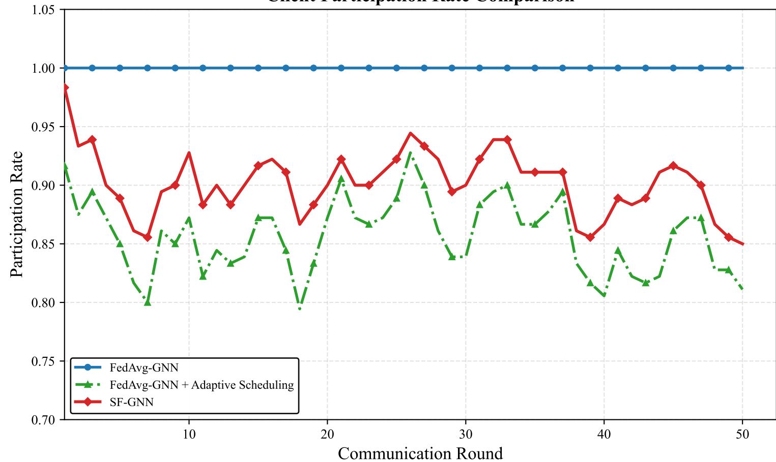
Client Participation Rate Comparison
