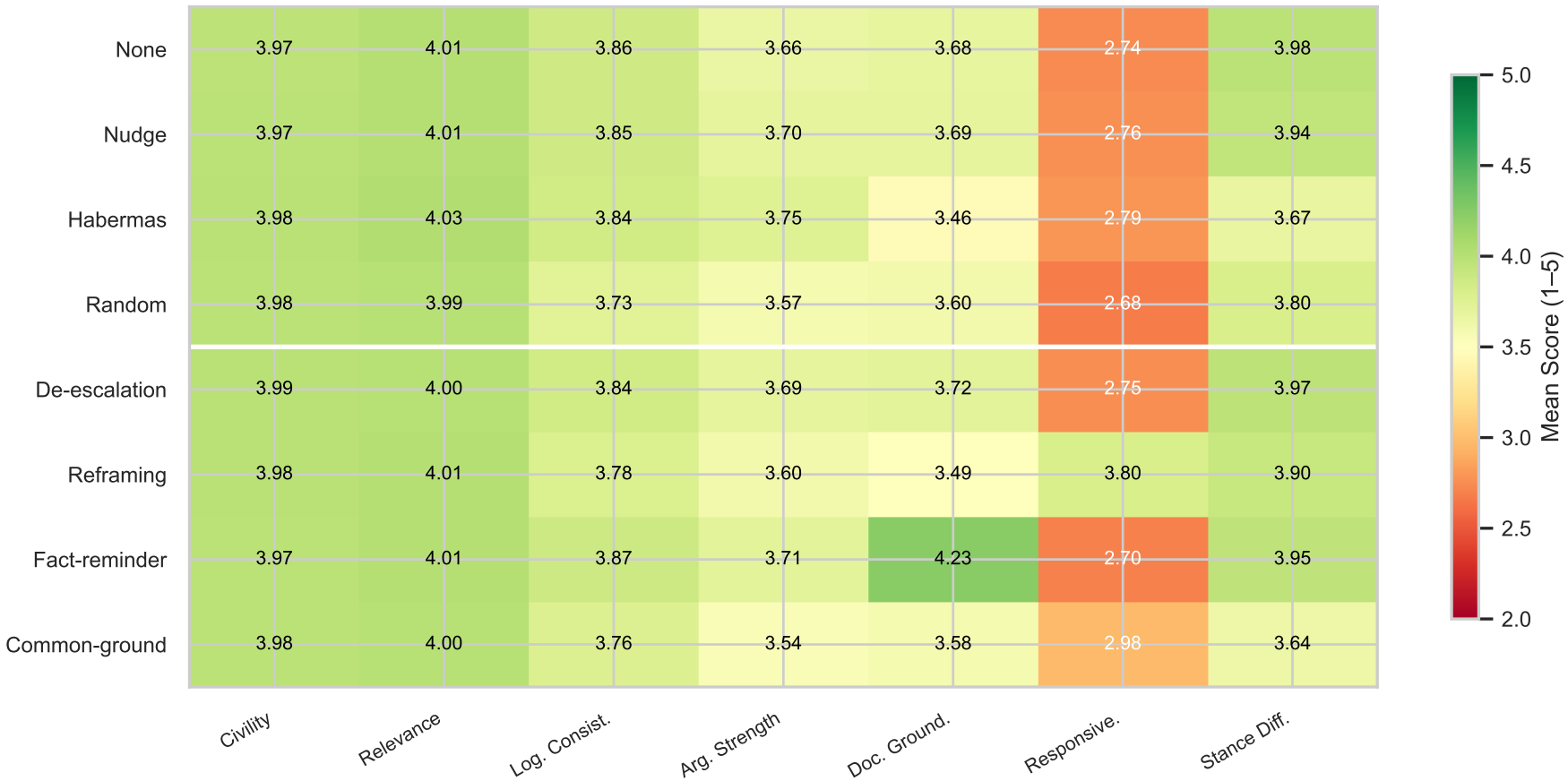
RQ2: Mean Discourse Quality Scores — Conditions × Dimensions
