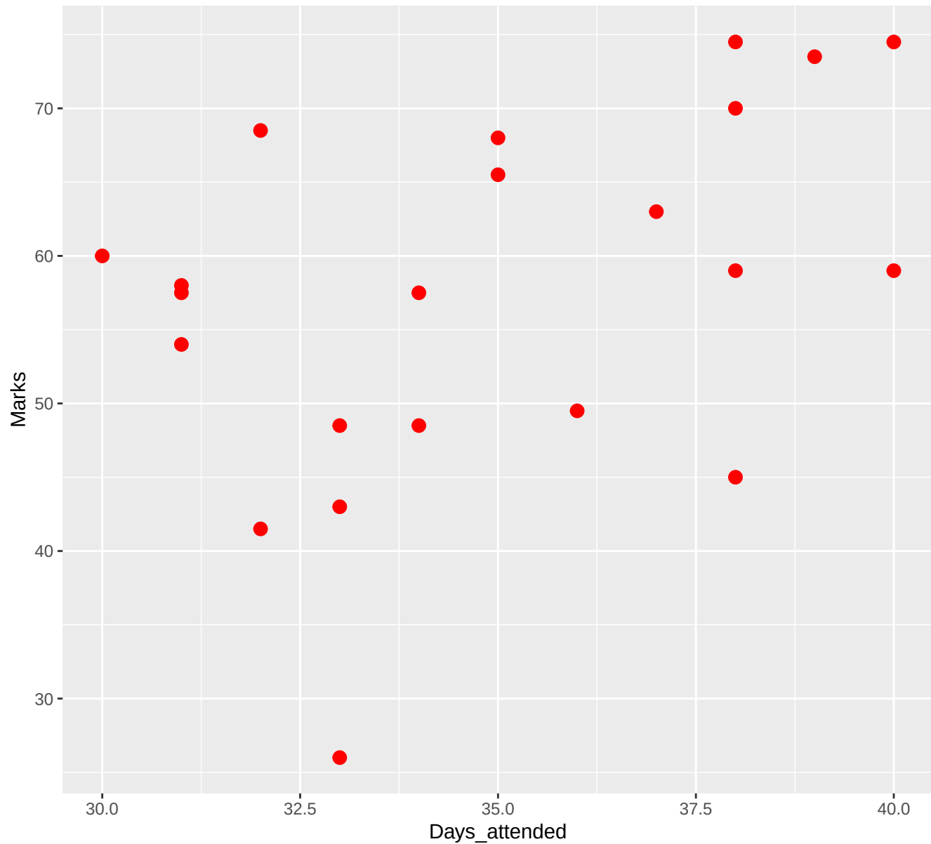
Scatter plot of number of days attended and marks by the students in MTech Data Science course (MA589)
