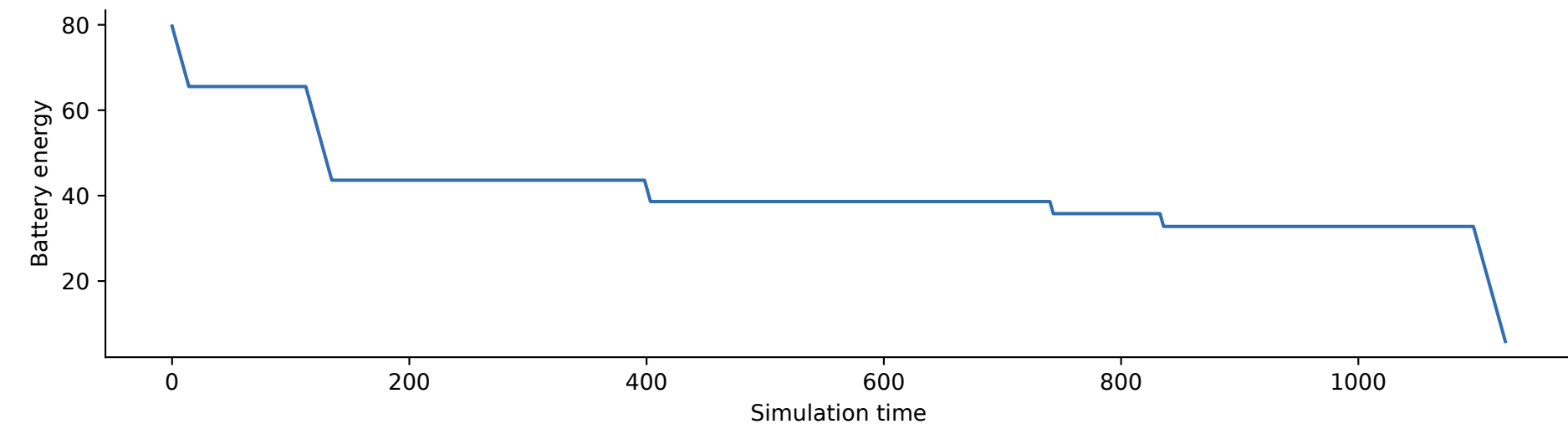
EV4: route with most served customers (lowest-ID tie break)
