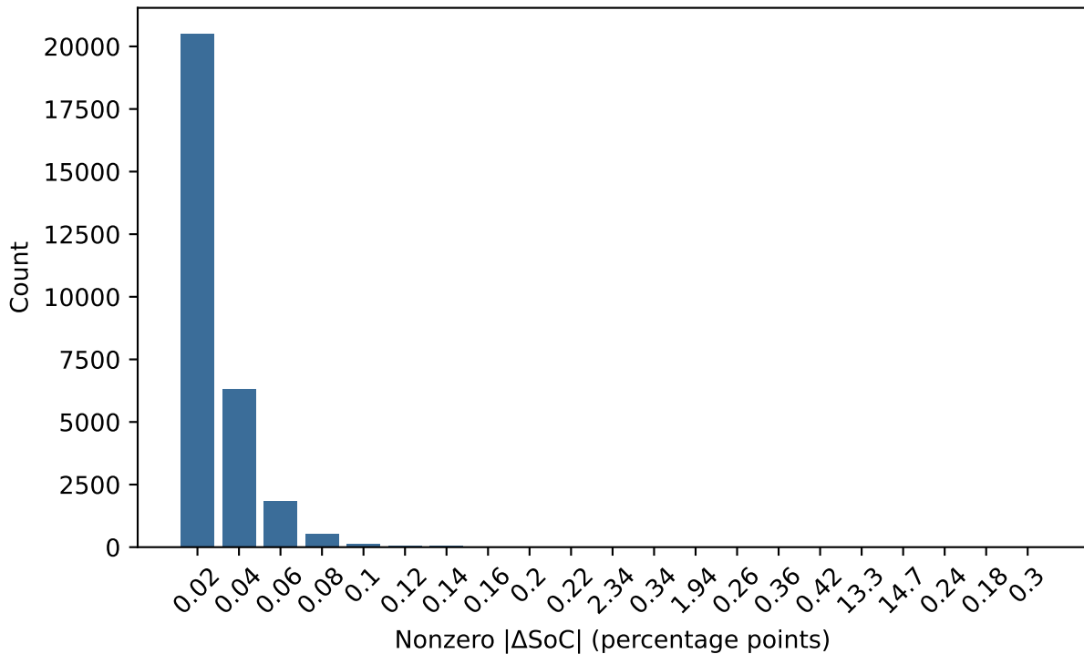
SoC transition distribution (estimated q = 0.02 )
