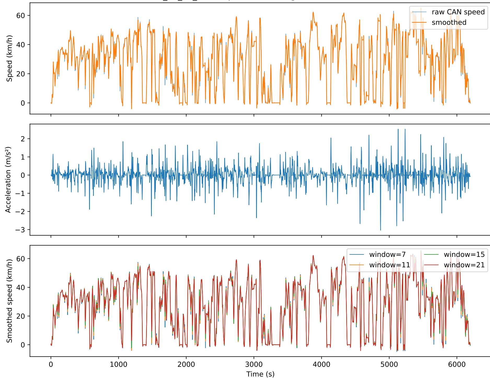
T1_03_29_2021: speed smoothing and acceleration
