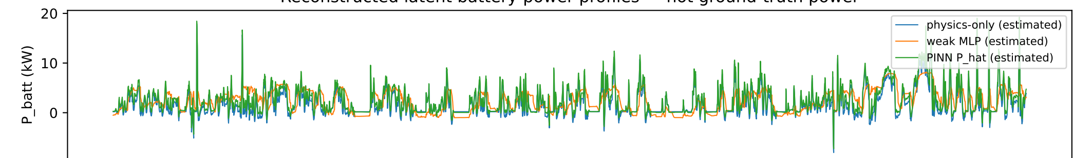
Reconstructed latent battery-power profiles — not ground-truth power
