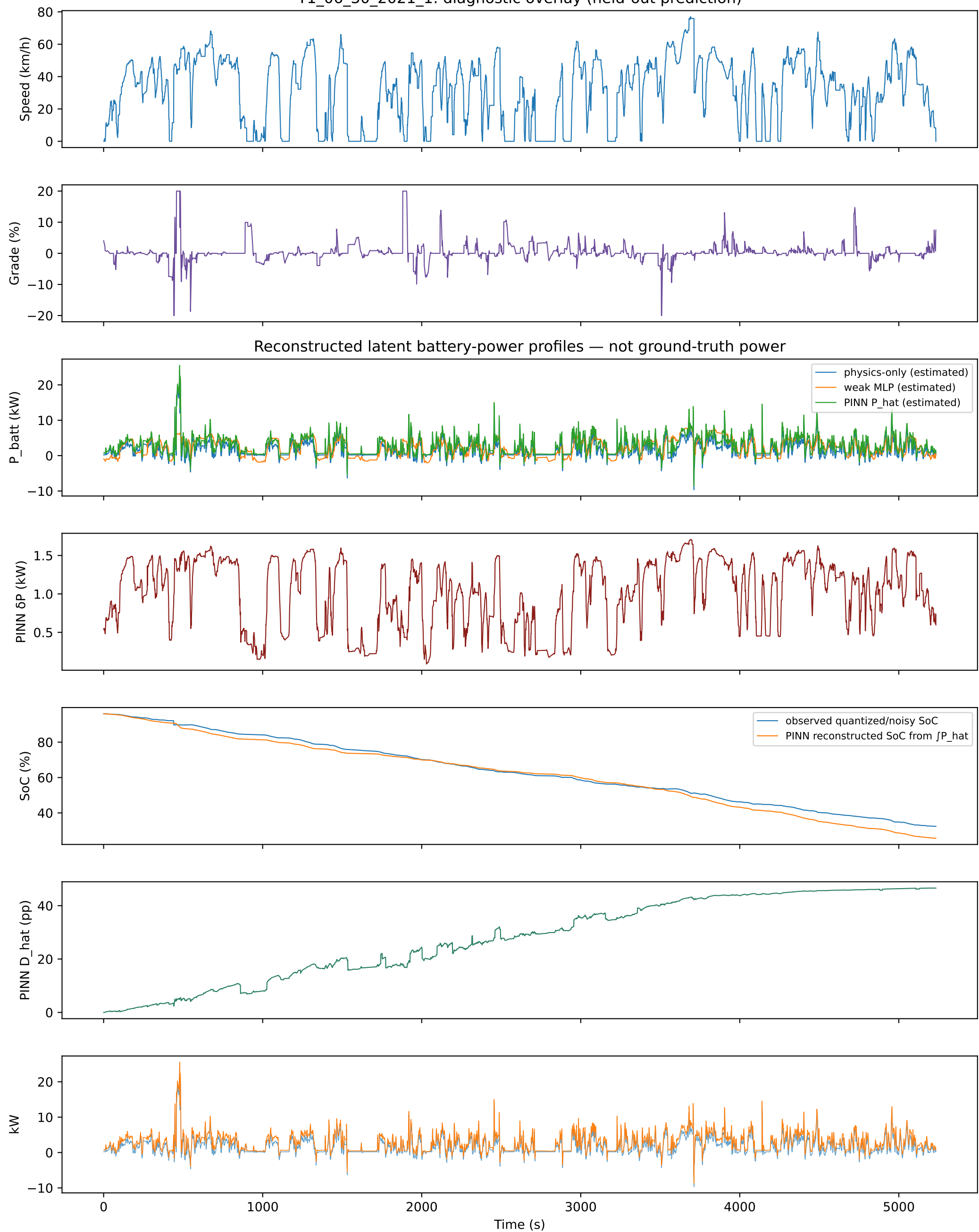
T1_06_30_2021_1: diagnostic overlay (held-out prediction)
