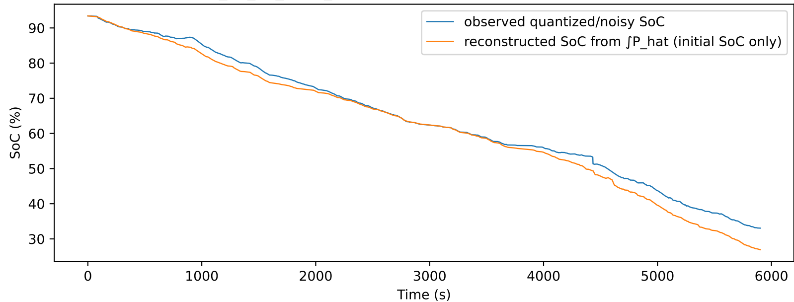
T1_06_30_2021_2: SoC reconstruction on an unseen trip
