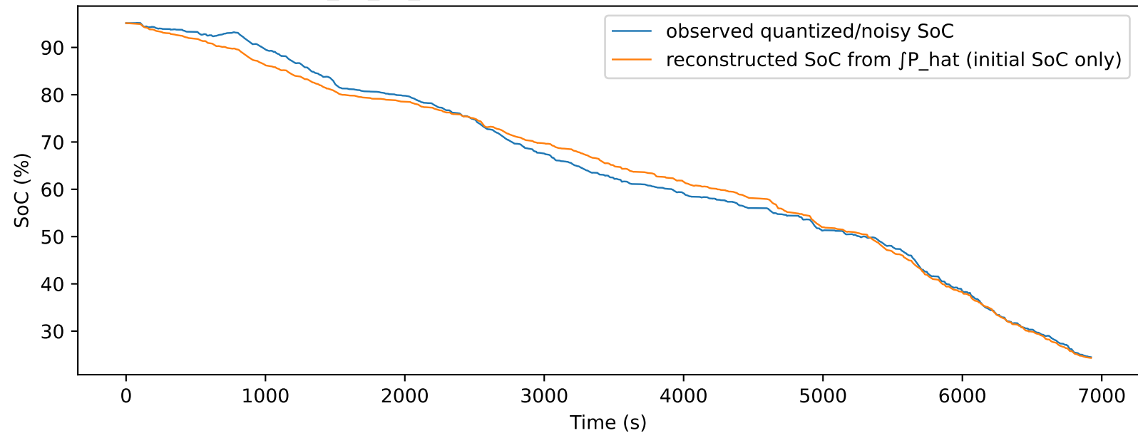
T2_03_30_2021: SoC reconstruction on an unseen trip
