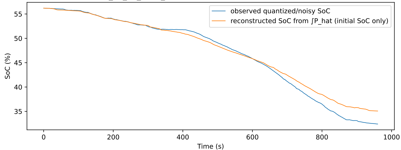
T3_05_25_2021_1: SoC reconstruction on an unseen trip
