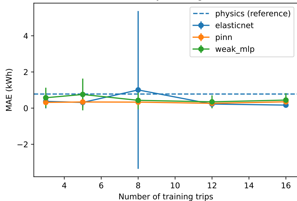
Data-scarcity learning curve
