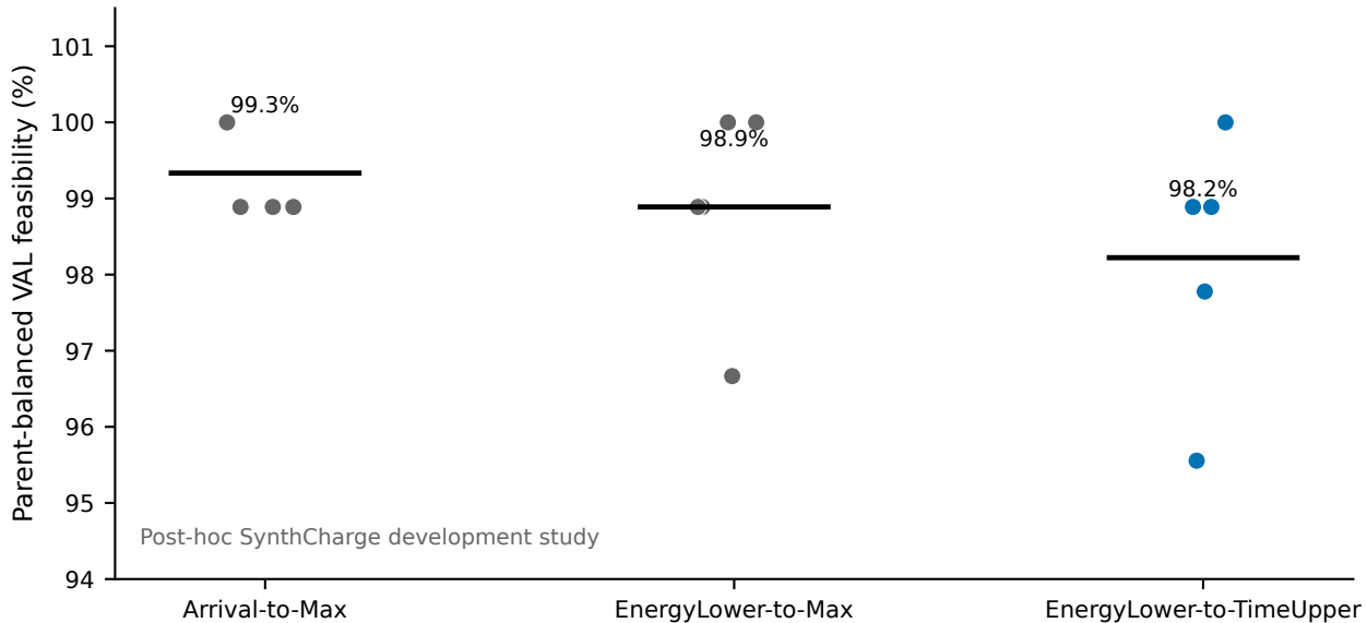
(a) Post-hoc SynthCharge development envelope study
