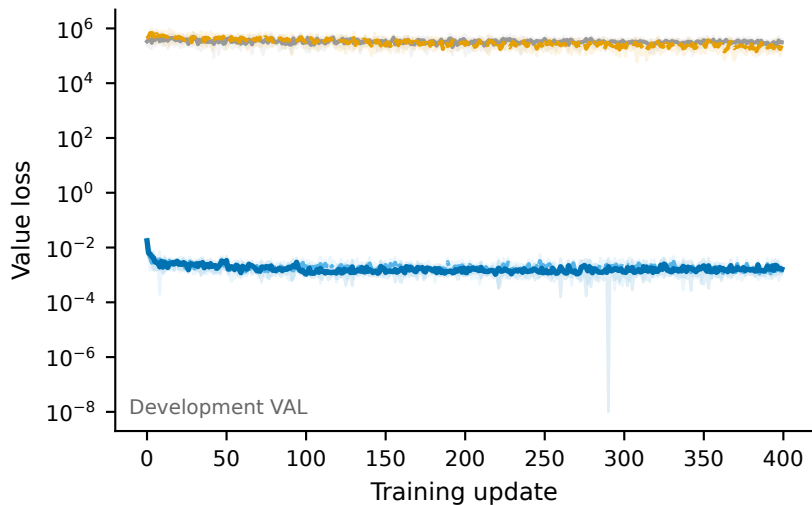
(a) Value loss
