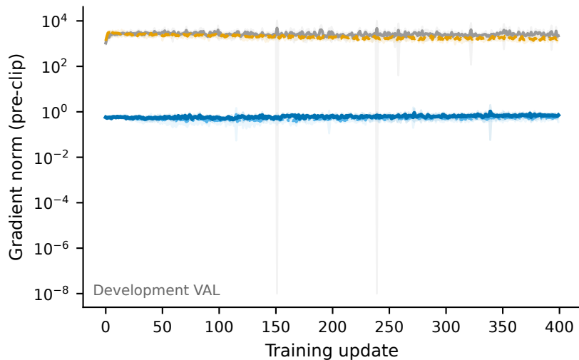
(b) Pre-clip gradient norm
