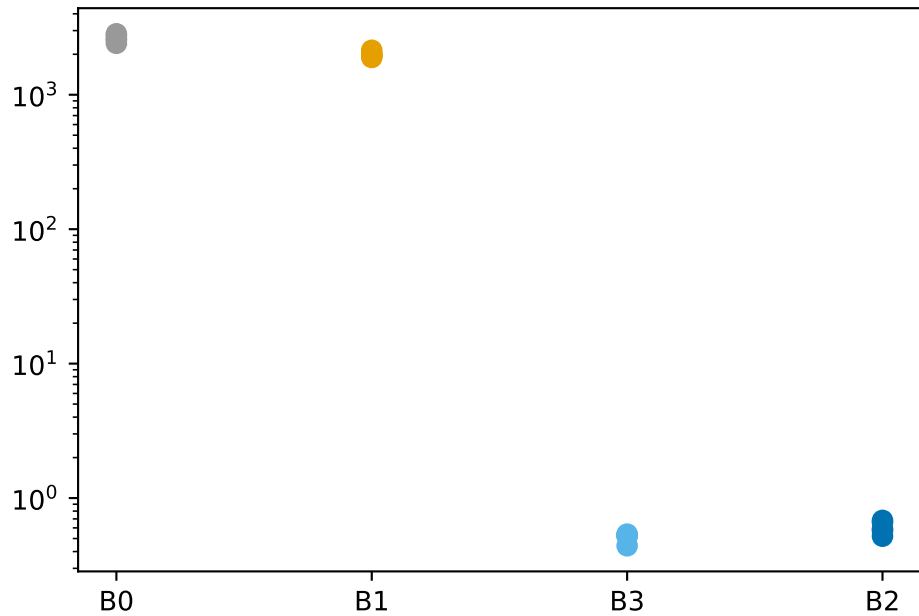
Mean grad norm (pre-clip)
