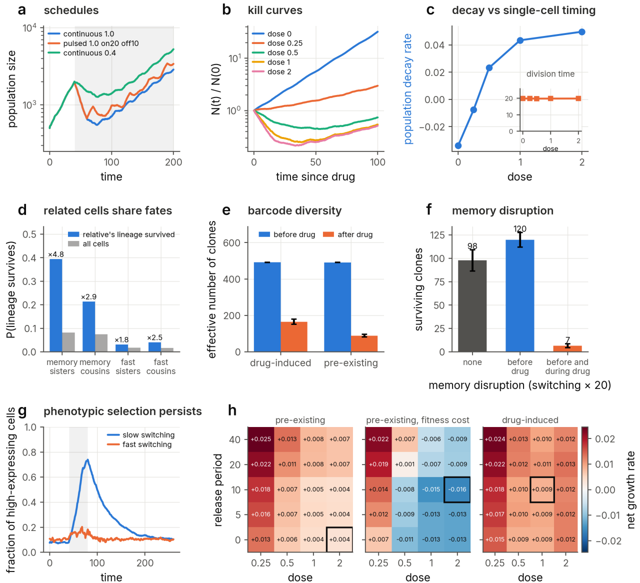
599 Fig. 4 | A single resistance gene with slow promoter switching reproduces persister biology. a, 600 Population size under continuous, pulsed and reduced-dose schedules (shading, treatment window). b, Kill curves 601 at increasing dose. c, Net population decay rate over the first 30 time units of treatment against dose, with 602 the mean division time of cells born under drug (inset), which is unchanged. d, Probability that a cell's lineage 603 survives the treatment (at least one descendant alive at the end of the run) given that its sister's or cousin's 604 lineage survived, against the marginal survival probability, for cells born in the 25 time units before the drug; 605 memory gene and fast-switching control, with the fold enrichment above each bar. e, Effective number of clones 606 (barcodes) before and after drug for pre-existing and drug-induced tolerance (mean \pm s.d. of three seeds). f, 607 Surviving clones after drug without memory disruption, with promoter switching accelerated 20-fold from two 608 cell-cycle times before the drug until the drug arrives, and with the acceleration maintained during exposure 609 (mean \pm s.d. of five seeds). g, Fraction of high-expressing cells before, during and after a drug pulse for slow 610 and fast switching. h, Net population growth rate over a 200-time-unit course as a function of release period 611 (time units without drug between 20-time-unit exposures) and dose, for pre-existing tolerance without and with a 612 fitness cost of the resistant state and for drug-induced tolerance; the box marks the most effective schedule.
