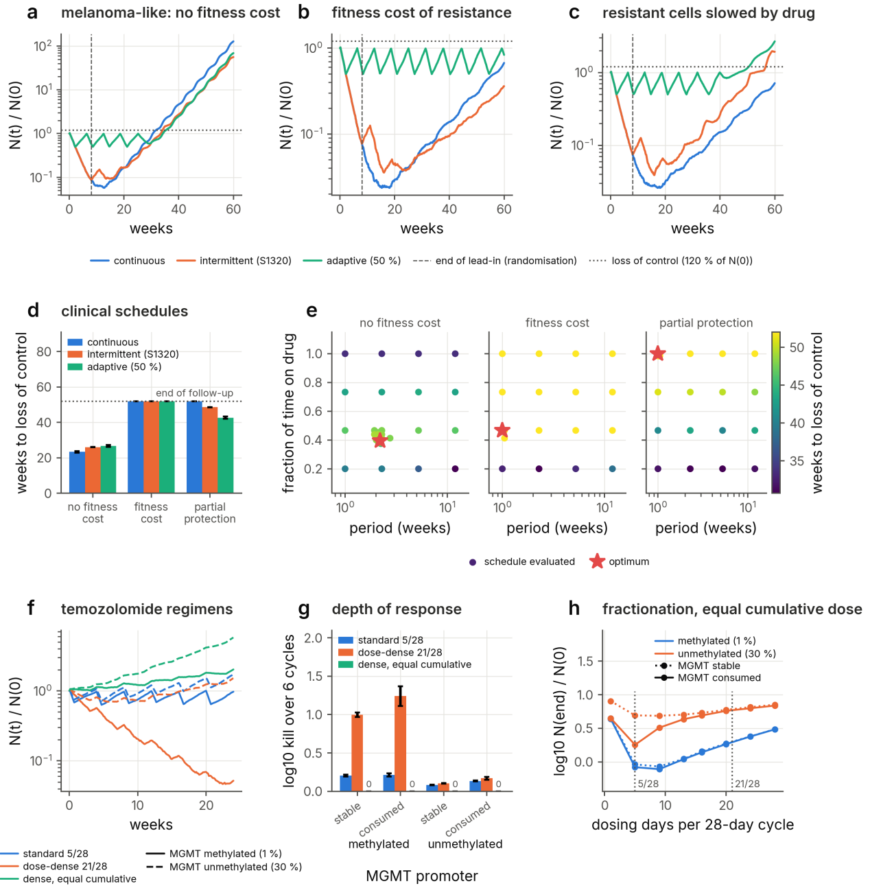
641 Fig. 8 | Dose and schedule optimisation against clinical regimens. a–c , Population size, relative to its 642 pre-treatment value, under continuous dosing, the intermittent schedule of the SWOG S1320 trial (8-week lead-in, 643 dashed line, then 3 weeks off and 5 weeks on) and adaptive therapy (drug withdrawn below 50% of the initial size, 644 resumed at the initial size) for a melanoma-like population with a rare, heritable pre-resistant state, when the 645 resistant state carries no fitness cost ( a ), when resistant cells grow 50% slower in the absence of drug ( b ), and 646 when resistant cells are only partly protected and grow at half speed under drug ( c ); dotted line, 120% of the 647 initial size. d , Weeks after randomisation until the population exceeds 120% of its pre-treatment size (loss of 648 control; mean \pm s.d. of four seeds, censored at 52 weeks). e , The same end point over intermittent schedules of 649 given period and fraction of time on drug after the lead-in, for every schedule evaluated by the optimiser (star, 650 best), for the three mechanisms.
