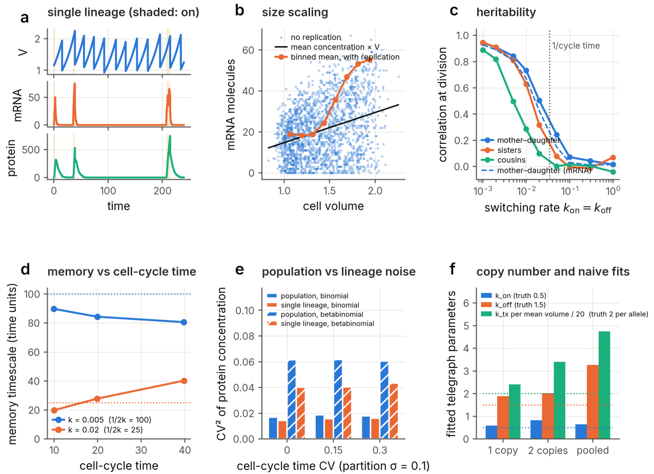
814 Fig. 3 | Growth, division and partitioning generate memory, size scaling and cell-cycle effects. a , A 815 single lineage: volume, mRNA and protein of a slowly switching gene, with the promoter-on state shaded. b , 816 mRNA count against cell volume for a fast-switching gene without replication (points; line, mean concentration 817 \times V ) and with gene replication at mid-cycle (binned means). c , Correlation at division between mothers 818 and daughters, sisters and cousins as a function of the promoter switching rate (protein concentration, solid; 819 mother-daughter mRNA, dashed); dotted line, inverse cell-cycle time. d , Memory timescale against the measured 820 cell-cycle time for two switching rates; dotted lines, 1/(k_{\text{on}} + k_{\text{off}}) . e , Squared coefficient of variation of a stable 821 protein's concentration across the population and along single lineages, for increasing partitioning noise and 822 cell-cycle-time noise. f , Telegraph parameters fitted to cells before replication (one gene copy), after replication 823 (two copies) and pooled. The transcription rate is plotted per unit cell volume and divided by twenty, so that all 824 three series share an axis and the dotted lines mark the true per-allele values ( k_{\text{on}} = 0.5 , k_{\text{off}} = 1.5 , and 2 for the 825 scaled transcription rate); the raw fitted transcription rates are in fig3f_copynumber.csv .
