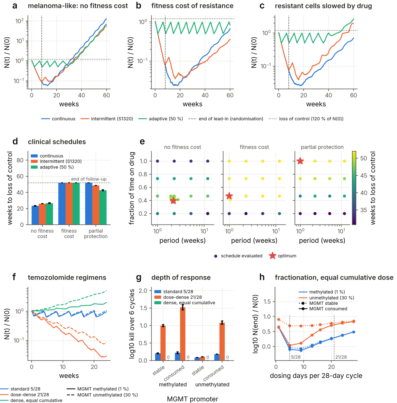
872 Fig. 8 | Dose and schedule optimisation against clinical regimens. a–c, Population size, relative to its 873 pre-treatment value, under continuous dosing, the intermittent schedule of the SWOG S1320 trial (8-week lead-in, 874 dashed line, then 3 weeks off and 5 weeks on) and adaptive therapy (drug withdrawn below 50% of the initial size, 875 resumed at the initial size) for a melanoma-like population with a rare, heritable pre-resistant state, when the 876 resistant state carries no fitness cost (a), when resistant cells grow 50% slower in the absence of drug (b), and 877 when resistant cells are only partly protected and grow at half speed under drug (c); dotted line, 120% of the 878 initial size. d, Weeks after randomisation until the population exceeds 120% of its pre-treatment size (loss of 879 control; mean \pm s.d. of four seeds, censored at 52 weeks). e, The same end point over intermittent schedules of 880 given period and fraction of time on drug after the lead-in, for every schedule evaluated by the optimiser (star, 881 best), for the three mechanisms. f, Population size under the standard (5 of 28 days) and dose-dense (21 of 28
