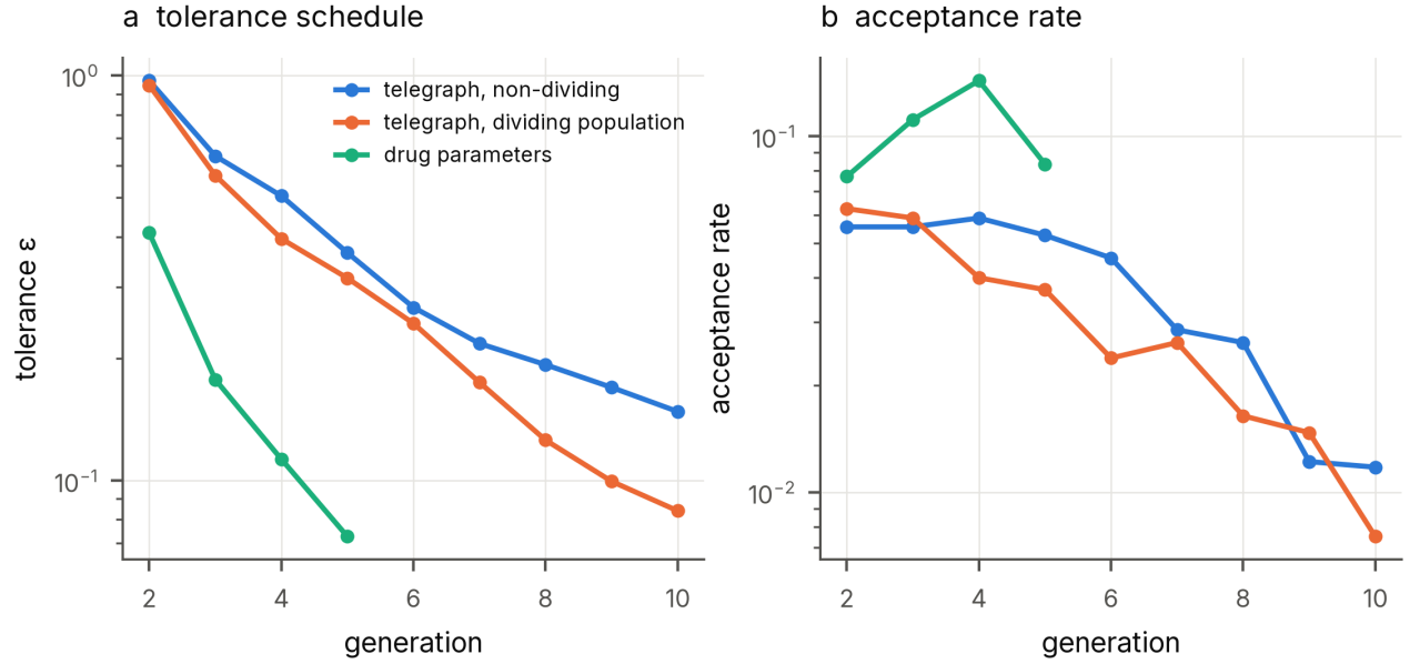
74 Supplementary Fig. 2 | ABC-SMC diagnostics. a , Tolerance and b , acceptance rate per generation for the 75 three runs of Fig. 6.
