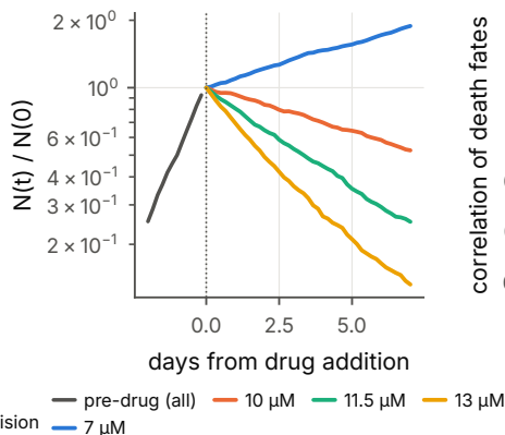
b predicted kill curves
