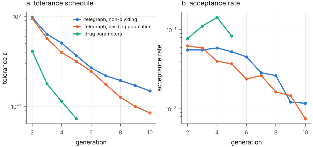
78 Supplementary Fig. 2 | ABC-SMC diagnostics. a , Tolerance and b , acceptance rate per generation for the 79 three runs of Fig. 6.
