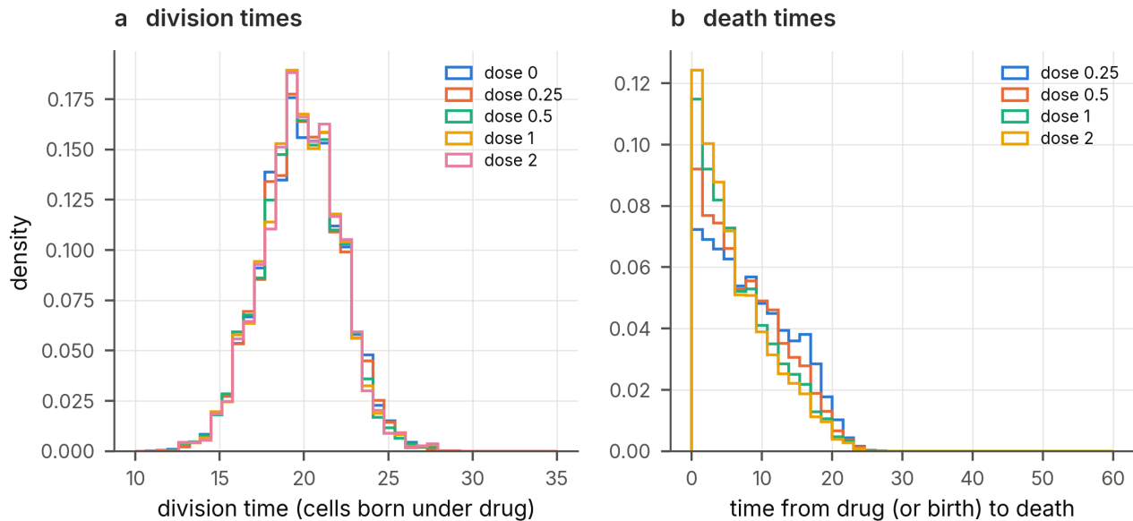
Supplementary Fig. 1 | Single-cell timing distributions underlying Fig. 4c. a , Division times of cells born under drug and b , times from drug start (or from birth, for cells born under drug) to death, per dose. The division-time distribution is set by the sizer and is the same at every dose, because in this model the drug kills but does not slow growth. Times to death are broad (coefficient of variation 0.72 at dose 0.5 and 0.82 at dose 2) and their mean shifts by much less than the population decay rate, because most deaths occur among low-expressing cells whose hazard is already close to h_{\max} at dose 0.5 ( EC_{50} = 0.5 , m = 2 ); raising the dose mainly shortens the survival of cells with intermediate protection. The dose dependence of population decay is therefore carried by the fraction of cells that are protected, not by the kinetics of death of unprotected cells, which is the interpretation 1 give of their single-cell tracking data. Under continuous dosing at the highest dose (release period 0, dose 2 in Fig. 4f), the long-term growth rate is
