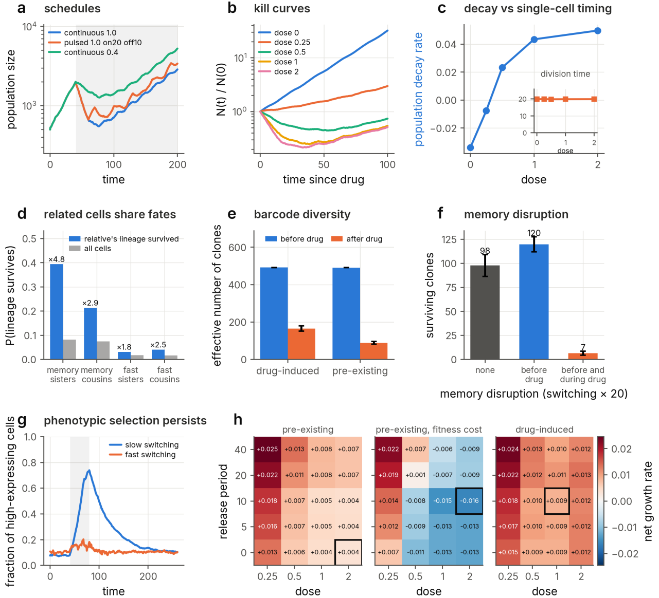
641 Fig. 4 | A single resistance gene with slow promoter switching reproduces persister biology. a , 642 Population size under continuous, pulsed and reduced-dose schedules (shading, treatment window). b , Kill curves 643 at increasing dose. c , Net population decay rate over the first 30 time units of treatment against dose, with 644 the mean division time of cells born under drug (inset), which is unchanged. d , Probability that a cell's lineage 645 survives the treatment (at least one descendant alive at the end of the run) given that its sister's or cousin's 646 lineage survived, against the marginal survival probability, for cells born in the 25 time units before the drug; 647 memory gene and fast-switching control, with the fold enrichment above each bar. e , Effective number of clones 648 (barcodes) before and after drug for pre-existing and drug-induced tolerance (mean \pm s.d. of three seeds). f , 649 Surviving clones after drug without memory disruption, with promoter switching accelerated 20-fold from two 650 cell-cycle times before the drug until the drug arrives, and with the acceleration maintained during exposure 651 (mean \pm s.d. of five seeds). g , Fraction of high-expressing cells before, during and after a drug pulse for slow 652 and fast switching. h , Net population growth rate over a 200-time-unit course as a function of release period 653 (time units without drug between 20-time-unit exposures) and dose, for pre-existing tolerance without and with a 654 fitness cost of the resistant state and for drug-induced tolerance; the box marks the most effective schedule.
