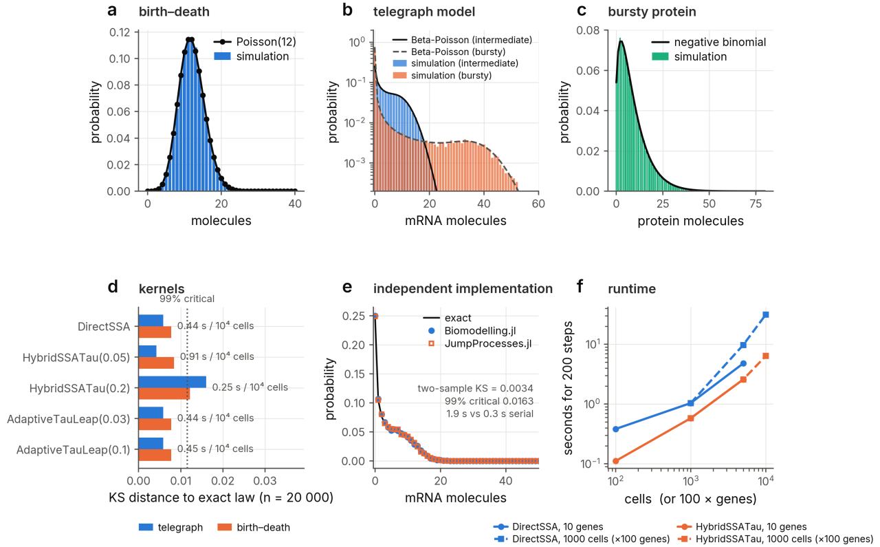
621 Fig. 2 | The engine matches exact laws and an independent implementation. a , Stationary distribution 622 of a birth-death process (bars, 50,000 simulated cells; line, Poisson law). b , Telegraph model in an intermediate 623 and a bursty regime against the Beta-Poisson law. c , Bursty protein production against the negative binomial. d , 624 Kolmogorov-Smirnov distance to the exact law for every kernel (n = 20,000; dotted line, 99% critical value) with 625 wall-clock time per 10^4 cells. e , Telegraph model simulated with Biomodelling.jl and with JumpProcesses.jl on 626 the same model; the two-sample Kolmogorov-Smirnov statistic lies below its 99% critical value. f , Runtime of 627 population simulations against the number of cells (10 genes) and genes (1,000 cells) for the exact and hybrid 628 kernels.
