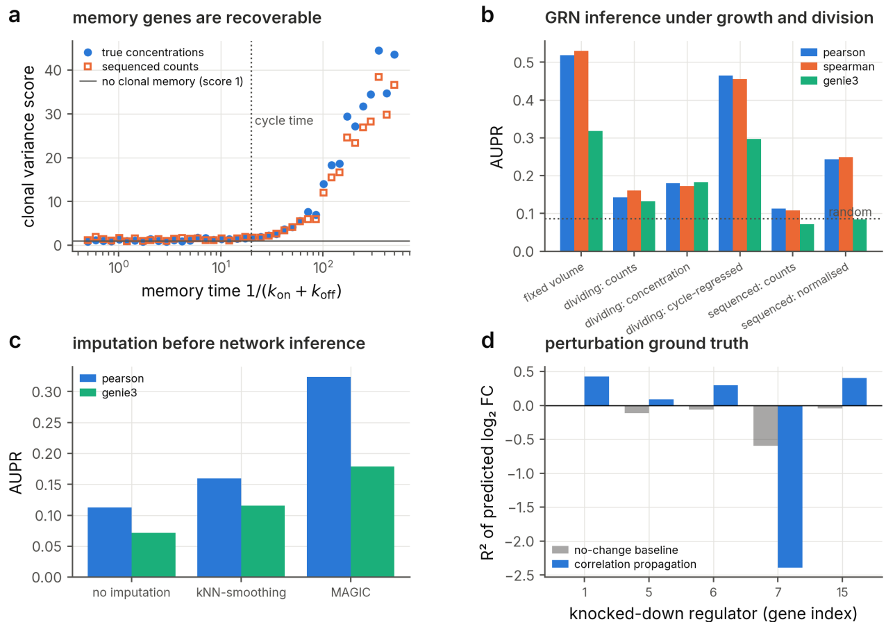
656 Fig. 5 | Ground-truth benchmarks. a , Clonal variance score against the known memory time of 40 657 independent genes, from true concentrations and from sequenced counts; dotted line, cell-cycle time. b , Area 658 under the precision-recall curve of correlation (Pearson, Spearman) and GENIE3 network inference on the same 659 30-gene network observed at fixed volume, in a dividing population (raw counts, concentrations, and concentrations 660 regressed on the cell-cycle covariates copy number and age) and after sequencing (raw and library-size normalised 661 counts); dotted line, random ranking. c , Effect of kNN-smoothing and MAGIC imputation before inference. d , 662 Coefficient of determination of predicted \log_2 fold changes after knocking down the five most connected regulators, 663 for a no-change baseline and for propagation of observational correlations.
