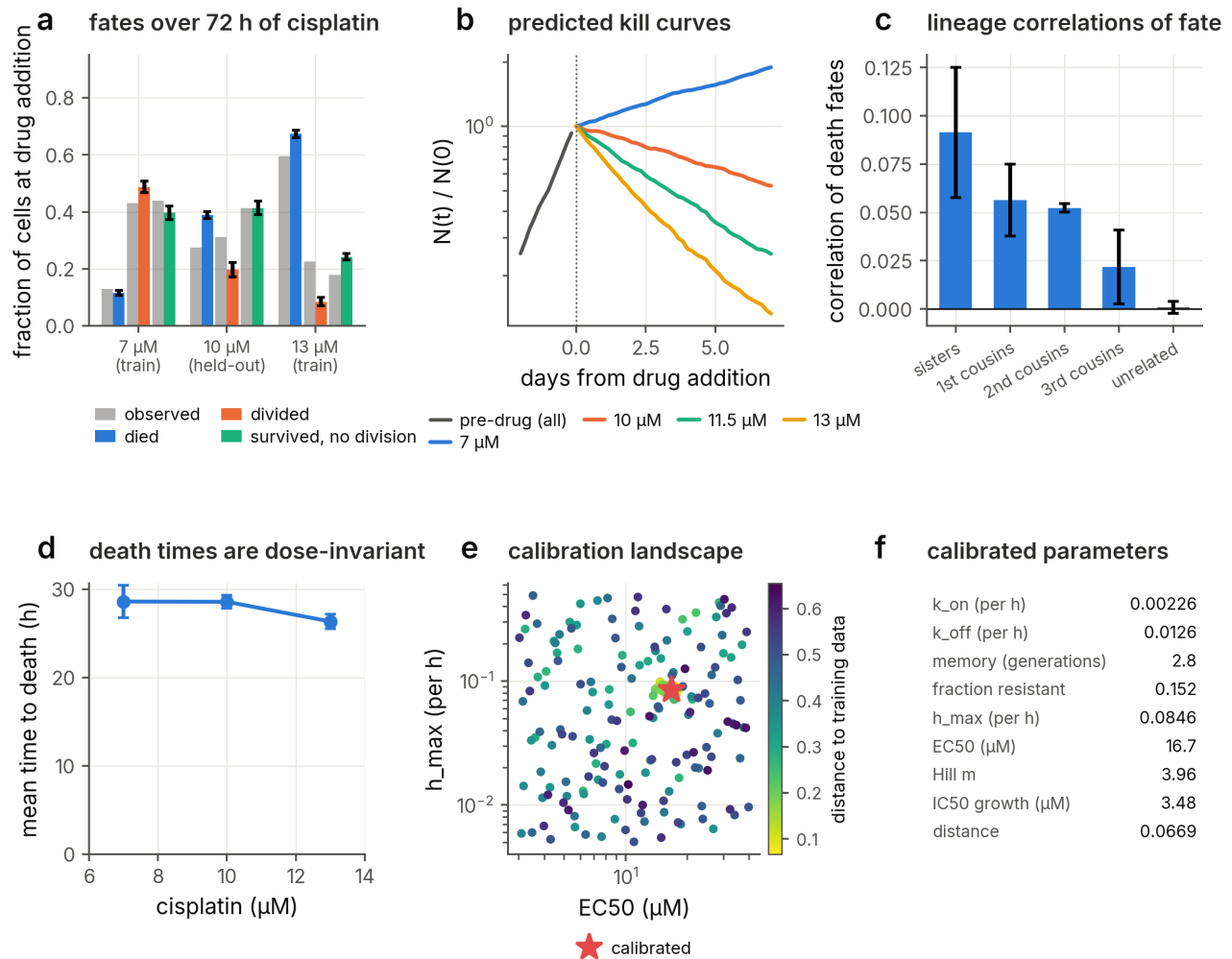
672 Fig. 7 | Calibration to laboratory time-lapse data and validation on held-out conditions. a , Fates 673 over 72 h of cisplatin of U2OS cells present at drug addition, observed by time-lapse microscopy (grey; ref. 6 ) and 674 simulated by the calibrated model (colours; mean \pm s.d. of four seeds); the model was calibrated on 7 and 13 \mu\text{M} 675 and the 10 \mu\text{M} condition is predicted. b , Predicted population size at the three concentrations and at 11.5 \mu\text{M} , 676 from two days before the drug to seven days of exposure. c , Correlation of death fates between sisters, first, second 677 and third cousins present at drug addition, and between unrelated cells (mean \pm s.d. of three seeds), against the 678 observation that correlations extend to second but not third cousins. d , Mean time to death of cells present at 679 drug addition against concentration (mean \pm s.d. of four seeds); division times are not shown because too few 680 cells born under drug divided again to estimate them (at most four per condition). e , Calibration landscape: every 681 parameter set evaluated by the optimiser, coloured by its distance to the training data. f , Calibrated parameters.
