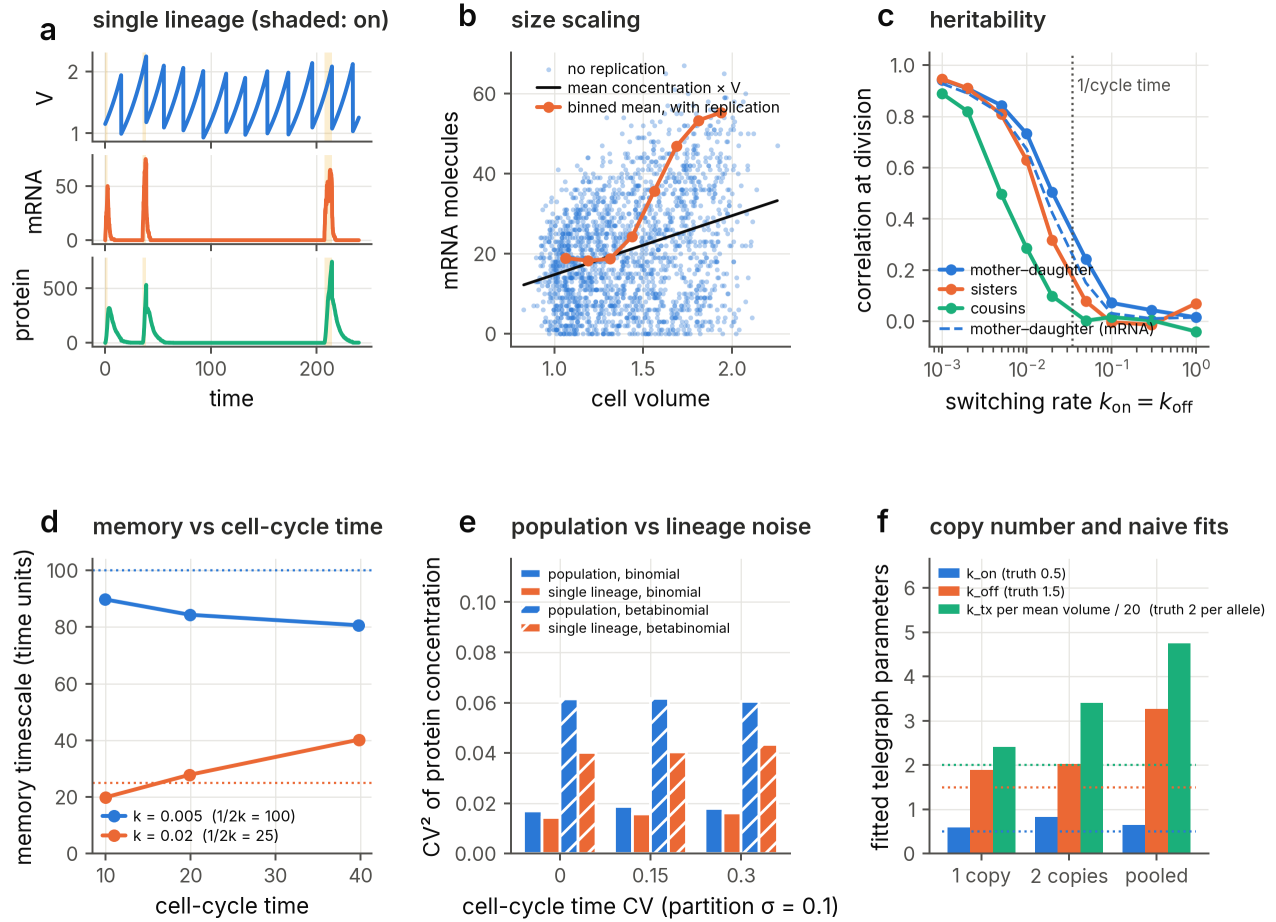
630 Fig. 3 | Growth, division and partitioning generate memory, size scaling and cell-cycle effects. a , A 631 single lineage: volume, mRNA and protein of a slowly switching gene, with the promoter-on state shaded. b , 632 mRNA count against cell volume for a fast-switching gene without replication (points; line, mean concentration 633 \times V ) and with gene replication at mid-cycle (binned means). c , Correlation at division between mothers 634 and daughters, sisters and cousins as a function of the promoter switching rate (protein concentration, solid; 635 mother-daughter mRNA, dashed); dotted line, inverse cell-cycle time. d , Memory timescale against the measured 636 cell-cycle time for two switching rates; dotted lines, 1/(k_{on} + k_{off}) . e , Squared coefficient of variation of a stable 637 protein's concentration across the population and along single lineages, for increasing partitioning noise and 638 cell-cycle-time noise. f , Telegraph parameters fitted to cells before replication (one gene copy), after replication 639 (two copies) and pooled; dotted lines, per-allele values.
