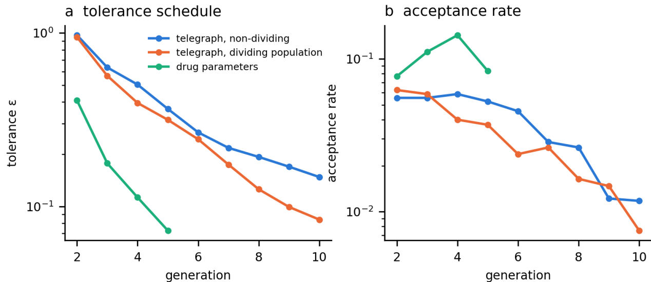
Figure S2. ABC-SMC diagnostics. (a) Tolerance and (b) acceptance rate per generation for the three runs of Figure 6.
