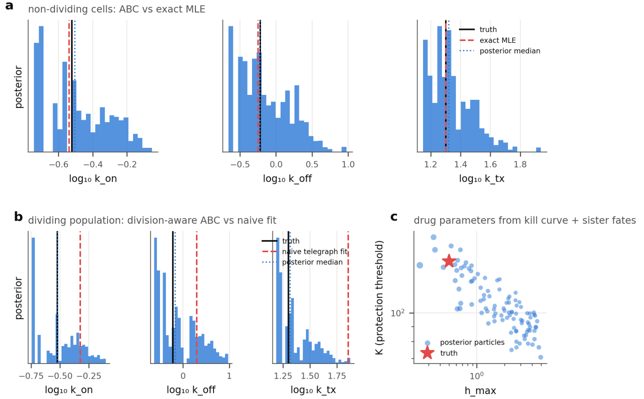
524 Fig. 6 | Inference with the forward model. a , Posterior distributions of telegraph parameters from ABC-SMC 525 on a snapshot of non-dividing cells, with the truth and the exact maximum-likelihood estimate. b , The same 526 for a snapshot of a growing and dividing population: the naive telegraph fit is biased while division-aware ABC 527 recovers the truth. c , Posterior particles for the maximal death rate and the protection threshold inferred from 528 a kill curve and sister fate concordance: the two parameters trade off along a ridge that contains the truth. d , 529 Posterior predictive kill curves simulated at the posterior median against the observed curve.
