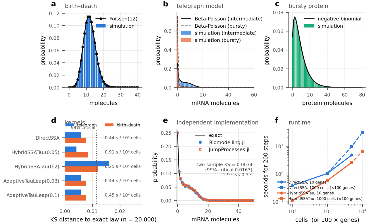
480 481 Fig. 2 | The engine is exact and agrees with an independent implementation. a , Stationary distribution 482 of a birth-death process (bars, 50,000 simulated cells; line, Poisson law). b , Telegraph model in an intermediate 483 and a bursty regime against the Beta-Poisson law. c , Bursty protein production against the negative binomial. d , 484 Kolmogorov-Smirnov distance to the exact law for every kernel (n = 20,000; dotted line, 99% critical value) with 485 wall-clock time per 10 4 cells. e , Telegraph model simulated with Biomodelling.jl and with JumpProcesses.jl on 486 the same model; the two-sample Kolmogorov-Smirnov statistic lies below its 99% critical value. f , Runtime of 487 population simulations against the number of cells (10 genes) and genes (1,000 cells) for the exact and hybrid 488 kernels.
