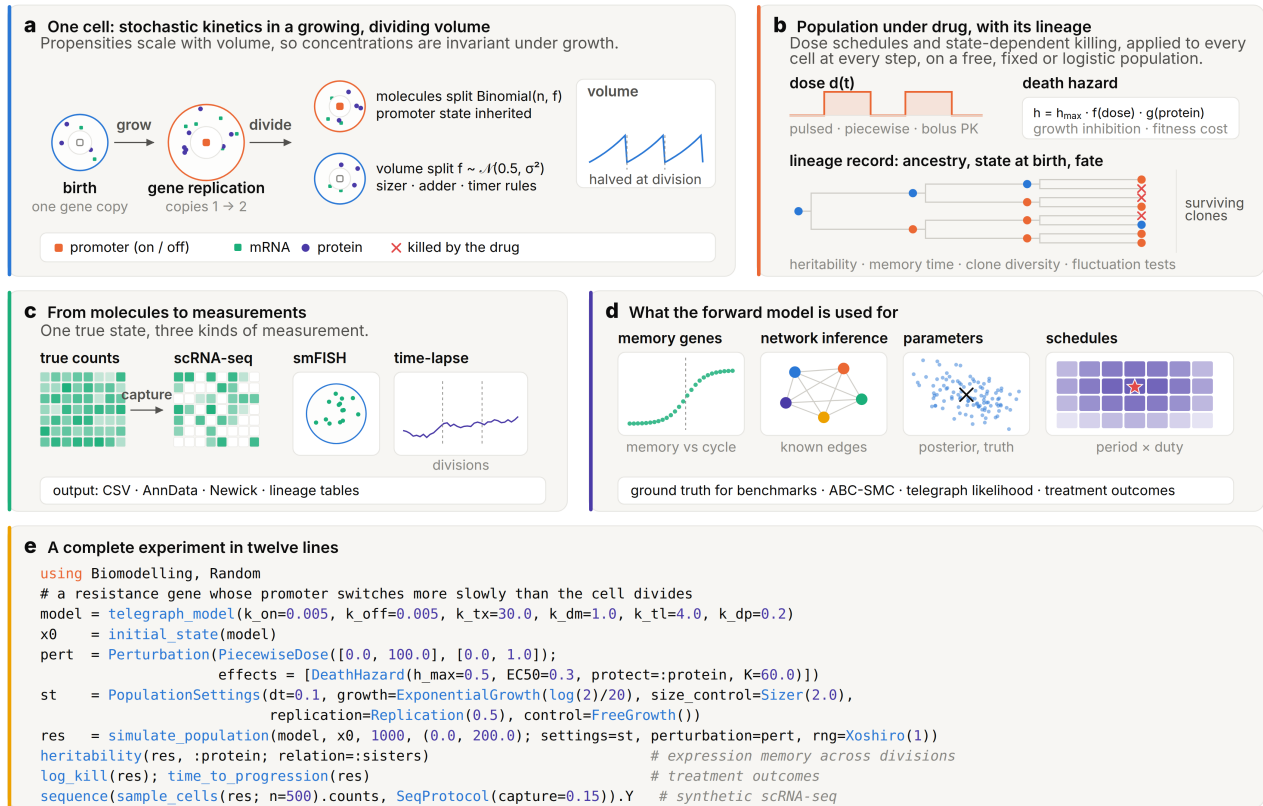
Fig. 1 | The Biomodelling.jl 2.0 framework. a, One cell. Reactions run at the cell's current volume, with propensities scaled so that concentrations are invariant under growth; genes replicate at a set point of the cycle;
