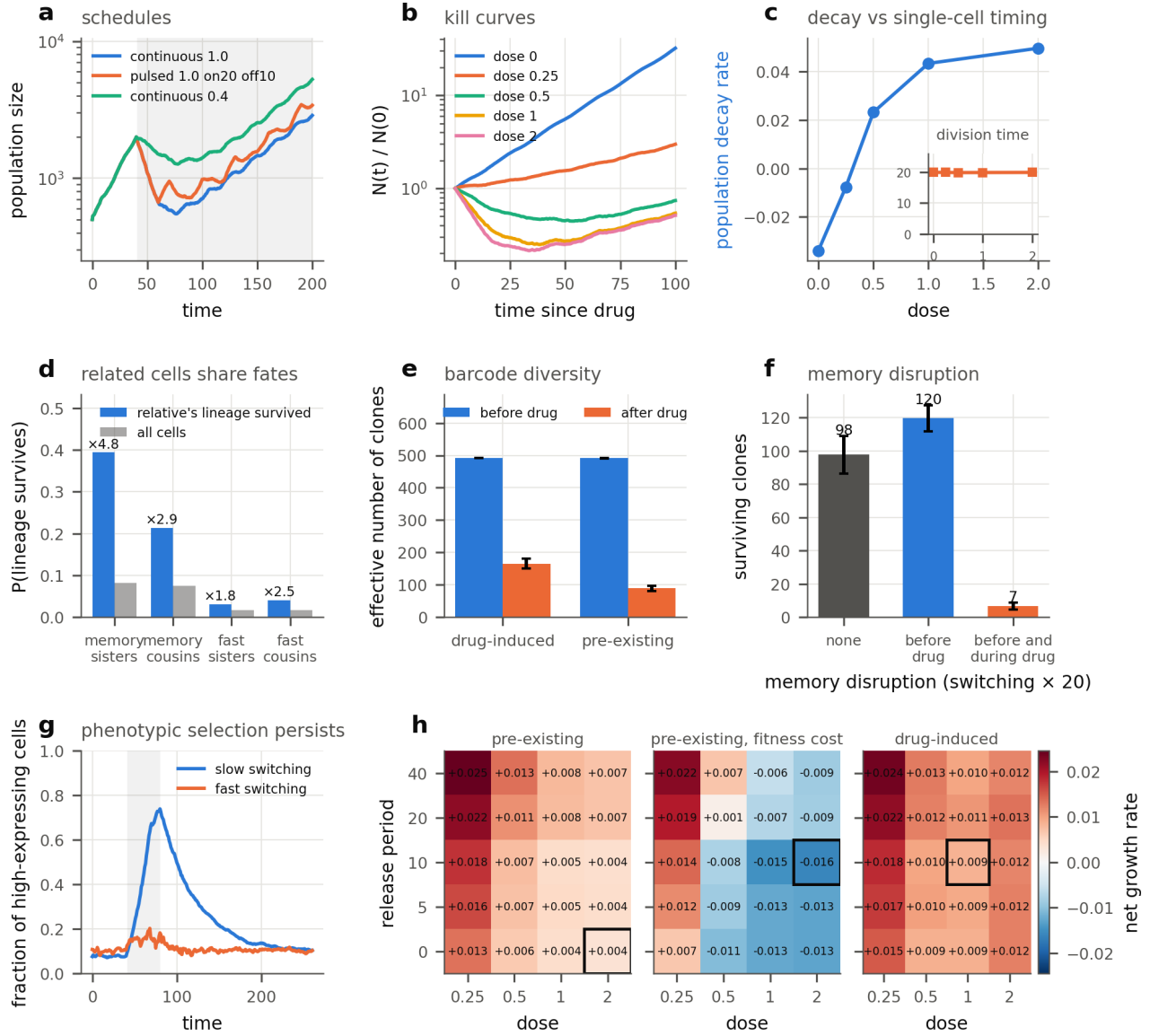
Figure 4. A single resistance gene with slow promoter switching reproduces persister biology. (a) Population size under continuous, pulsed and reduced-dose schedules (shading: drug present). (b) Kill curves at increasing dose. (c) Net population decay rate over the first 30 time units of treatment against dose, with the mean division time of cells born under drug (inset), which is unchanged. (d) Probability that a cell's lineage survives the treatment (at least one descendant alive at the end of the run) given that its sister's or cousin's lineage survived, against the marginal survival probability, for cells born in the 25 time units before the drug; memory gene and fast-switching control, with the fold enrichment above each bar. (e) Effective number of clones (barcodes) before and after drug for pre-existing and drug-induced tolerance (mean \pm s.d. of three seeds). (f) Surviving clones after drug without memory disruption, with promoter switching accelerated 20-fold from two cell-cycle times before the drug until the drug arrives, and with the acceleration maintained during exposure (mean \pm s.d. of five seeds). (g) Fraction of high-expressing cells before, during and after a drug pulse for slow and fast switching (MGMT-like phenotypic selection). (h) Net population growth rate over a 200-time-unit course as a function of release period (time units without drug between 20-time-unit exposures) and dose, for pre-existing tolerance without and with a fitness cost of the resistant state and for drug-induced tolerance; the box marks the
