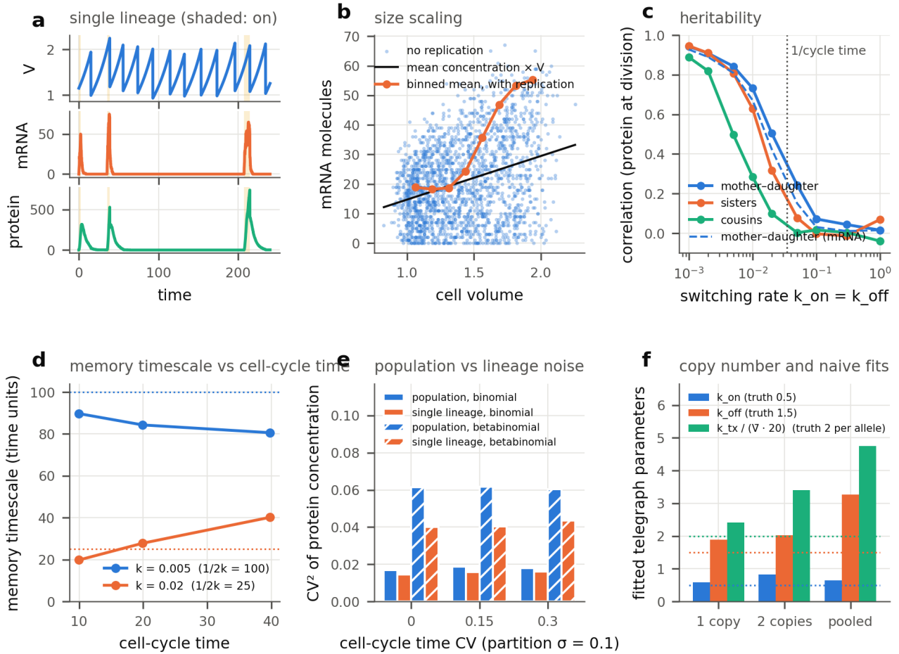
345 Figure 3. Growth, division and partitioning generate memory, size scaling and cell-cycle effects. (a) 346 A single lineage: volume, mRNA and protein of a slowly switching gene, with the promoter-on state shaded. (b) 347 mRNA count against cell volume for a fast-switching gene without replication (points, line: mean concentration 348 \times V ) and with gene replication at mid-cycle (binned means). (c) Correlation of protein concentration at division 349 between mothers and daughters, sisters and cousins as a function of the promoter switching rate; dotted: one over 350 the cell-cycle time. (d) Memory timescale in time units against the measured cell-cycle time for two switching 351 rates; dotted lines: 1/(k_{\text{on}} + k_{\text{off}}) . (e) Coefficient of variation squared of a stable protein's concentration 352 across the population and along single lineages, for increasing partitioning noise and cell-cycle-time noise. (f) 353 Telegraph parameters fitted to cells before replication (one gene copy), after replication (two copies) and pooled; 354 dotted: per-allele values.
